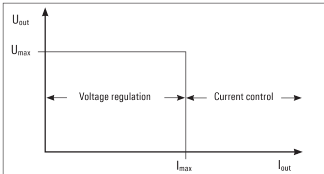
Fig. 4.5: Current limit
