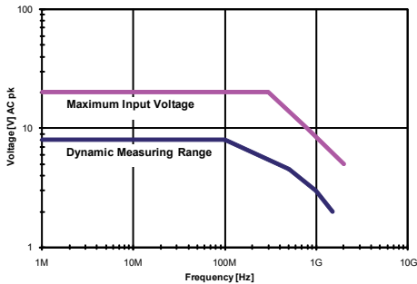
Input Voltage vs. Frequency
