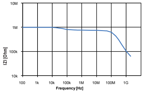
Typical Input Impedance
