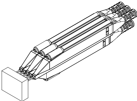
The HZ030 testing adjacent pins in 2.54 mm Pitch
