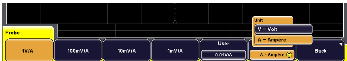
Figure 3-7: RTM Channel1 Probe Menu for RT-ZC10
