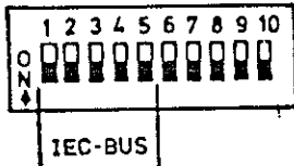
Fig. 2-6 Coding switch.
