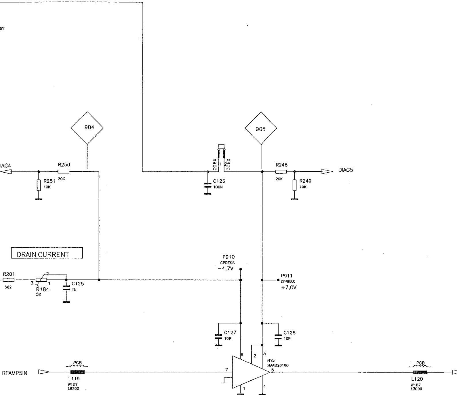
RF AMPLIFIER 5
