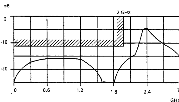
Fig. 5-5 |S11| Typical curve and tolerance field
