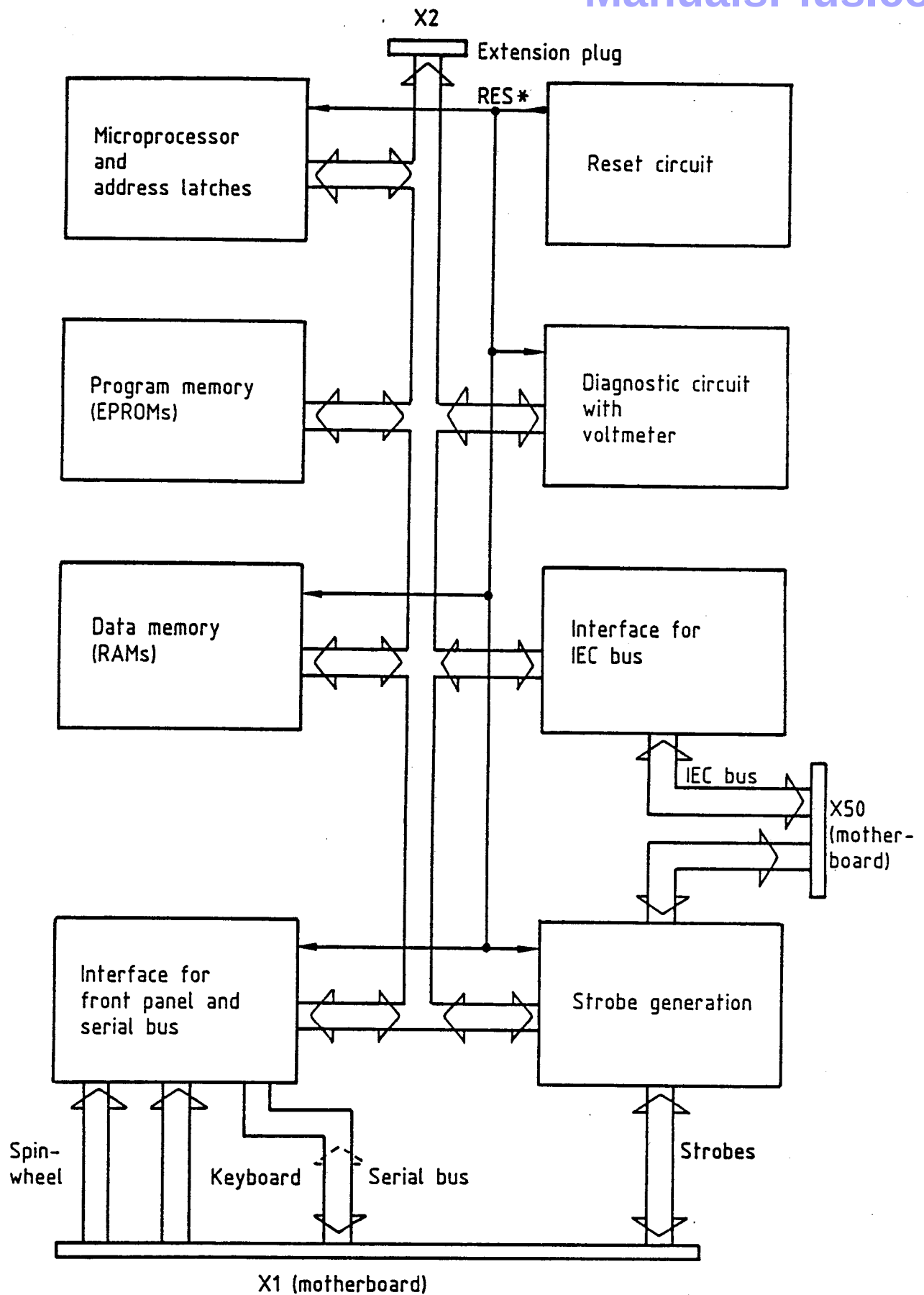
Fig. 5-4 Block diagram of processor
