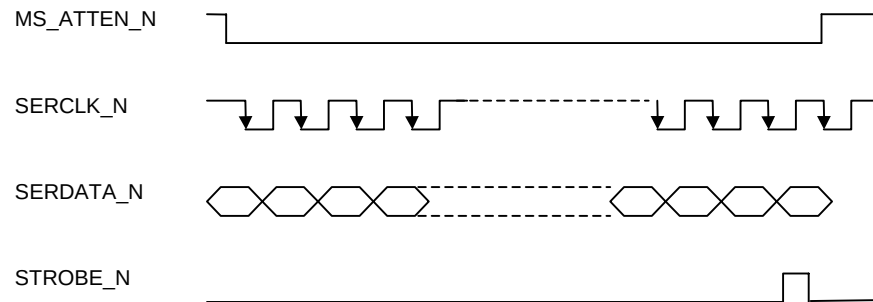
Fig. 3-1 Programming of attenuator, timing at interface X301.
