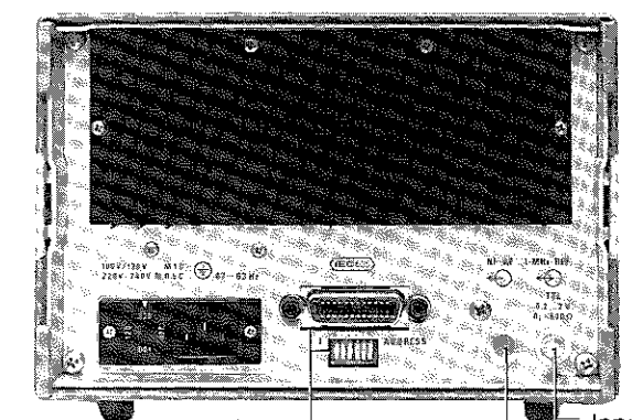
IEC-bus connector and address switch
