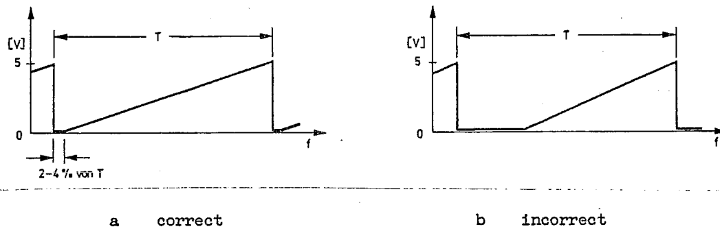
Fig. 6 Adjusting the Differential Amplifier T4-T5
