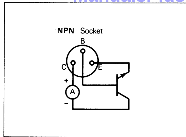
Fig. 12. Field calibration, f_r circuit.
