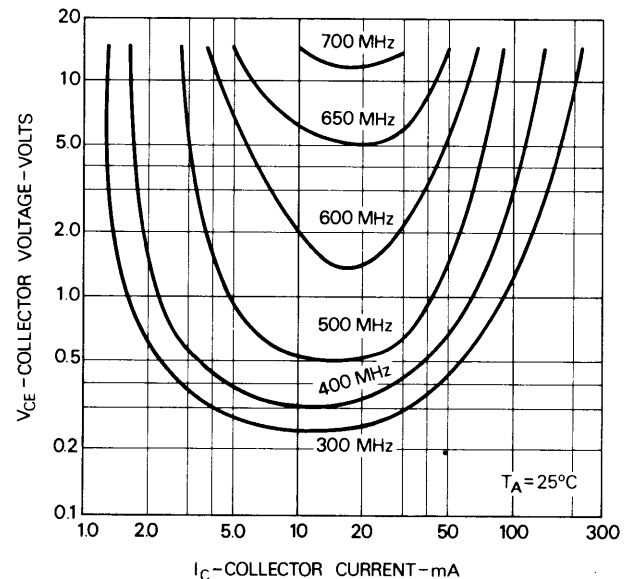
Fig. 16. Constant f_T curves for collector-emitter voltage vs. collector current (bipolar transistors).
