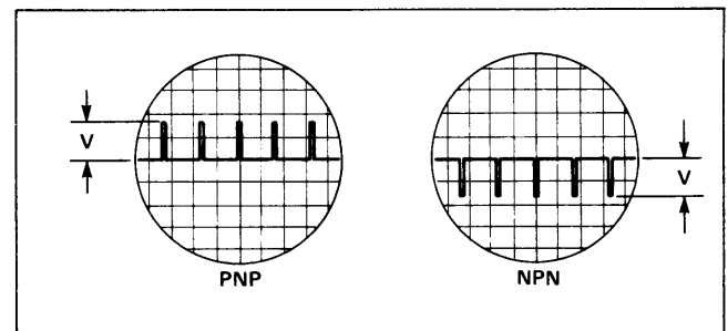
Fig. 10. Pulse voltage waveforms.
