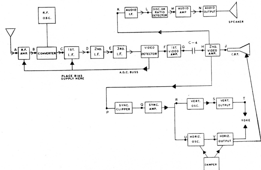
Figure 4—Block diagram of typical TV receiver
