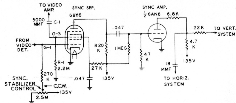
Figure 10 Sync Separator System
