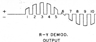
Figure 20—(R-Y) demodulator output as seen on an oscilloscope
