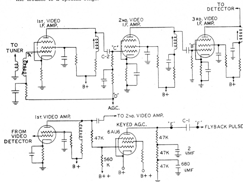
Figure 12—Video I.F. system and Keyed A.G.C. circuit
