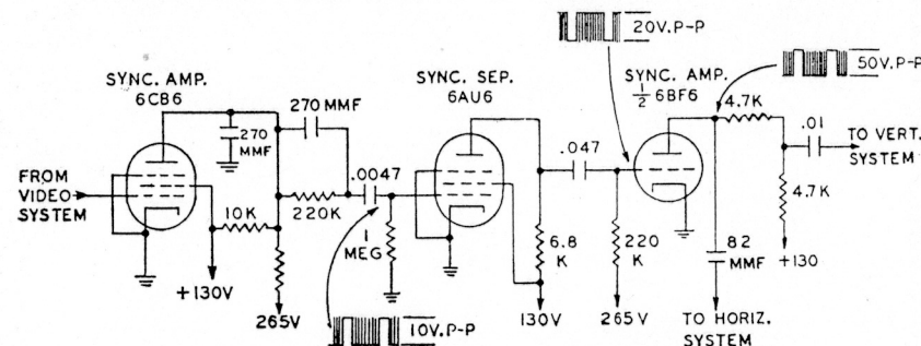
Figure 9—A more elaborate sync separator system
