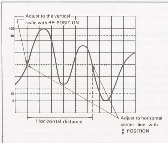
Fig. 7. Time Measurement.
