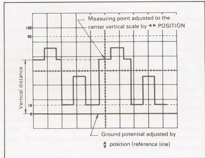
Fig. 5. DC Voltage Measurement.
