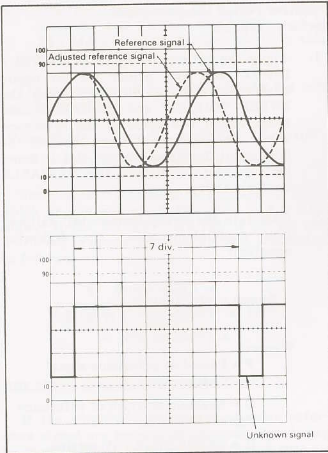
Fig. 12. Period Measurement, Relative Method.
