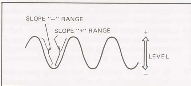
Fig. 4. Function of Slope and Level Controls.
