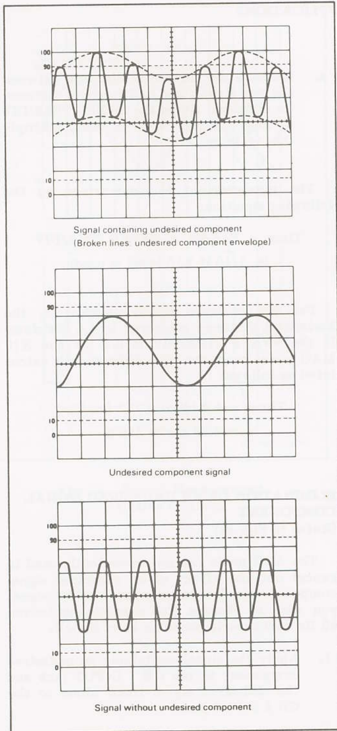
Fig. 14. Eliminating An Undesired Signal Component.
