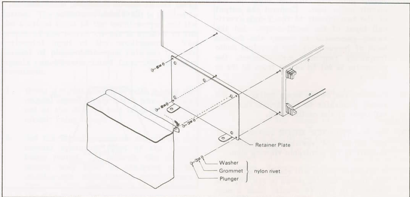
Fig. 21. Installation of LC-150 Probe Pouch.
