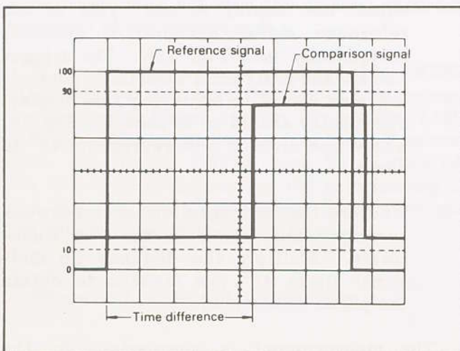
Fig. 13. Time Difference Measurement.
