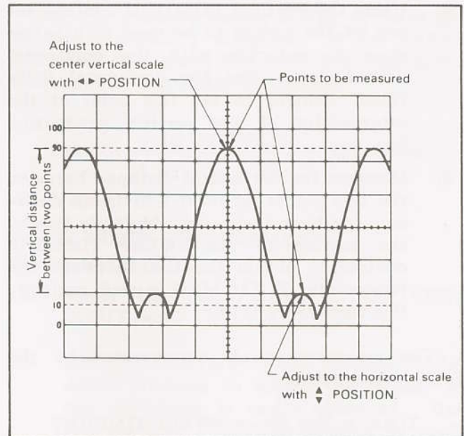
Fig. 6. Voltage Measurement.
