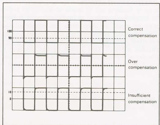
Fig. 22. Probe Compensation Adjustment.
