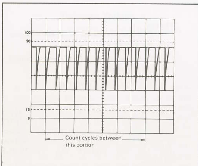
Fig. 9. Alternate Method of Frequency Measurement.
