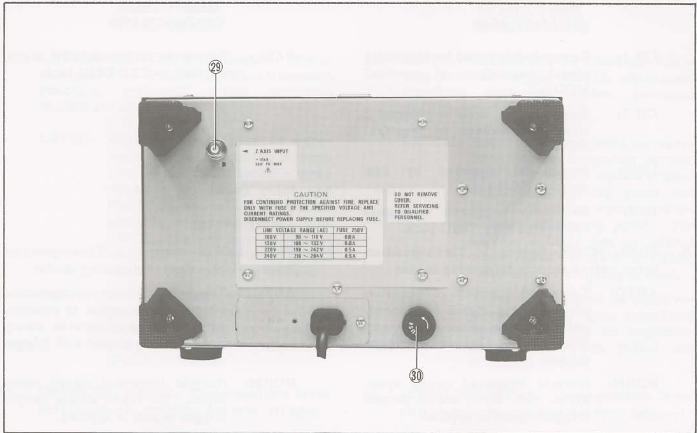
Fig. 2. Rear Panel Controls and Indicators.
