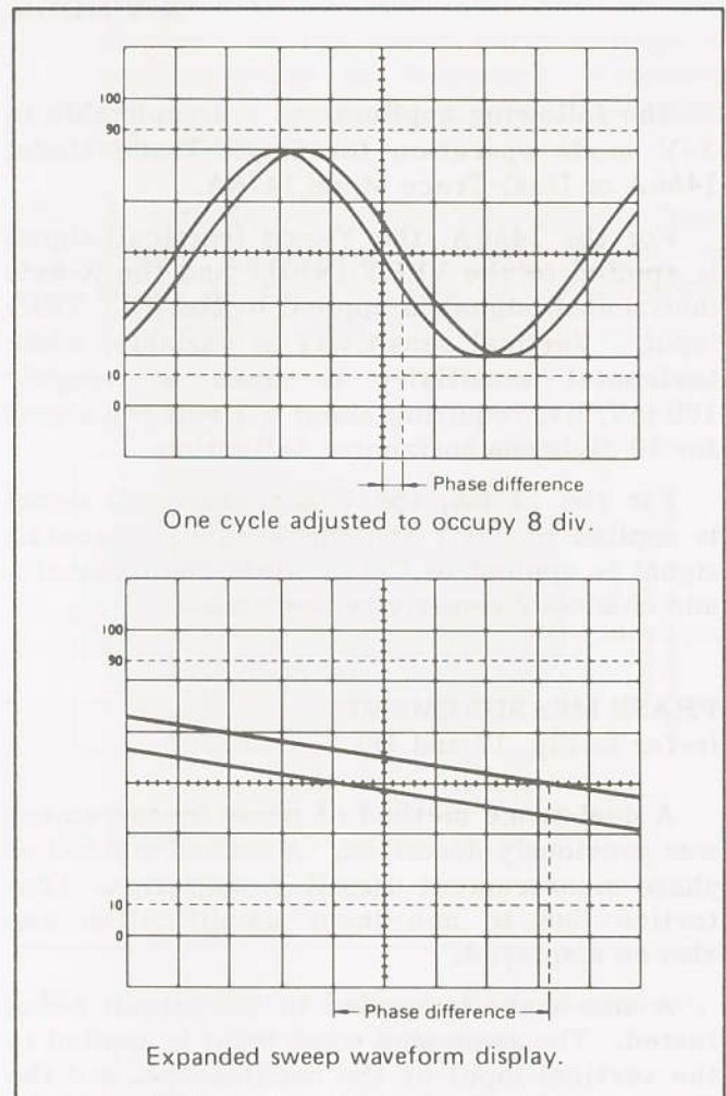
Fig. 16. Measuring Small Phase Difference.
