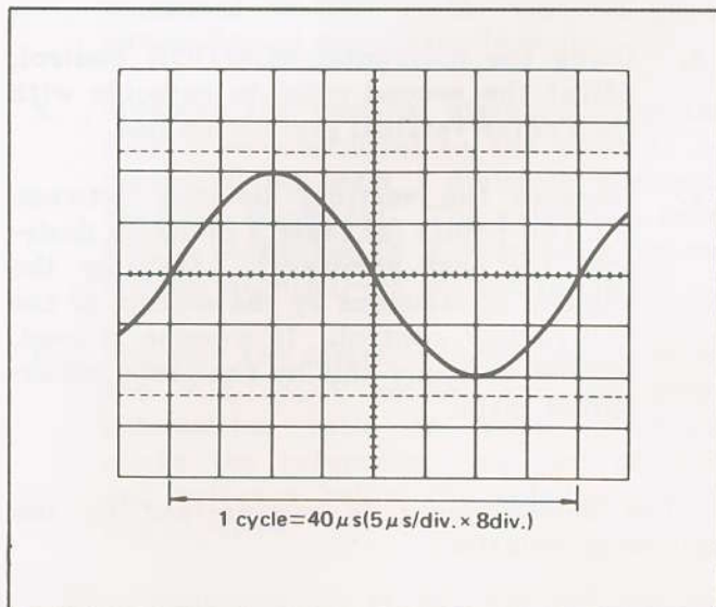
Fig. 8. Frequency Measurement.
