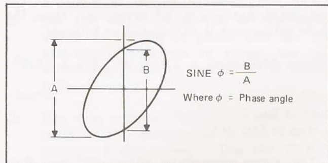
Fig. 18. Phase Measurement, X-Y Operation.
