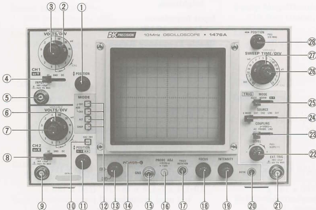
Fig. 1. Front Panel Controls and Indicators.
