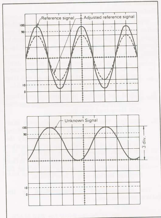
Fig. 11. Voltage Measurement, Relative Method.
