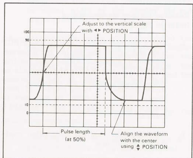
Fig. 10. Pulse Width Measurement.
