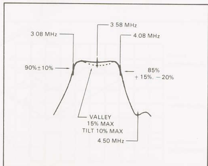
Fig. 20. Frequency Response Measurement, Demodulated Response.
