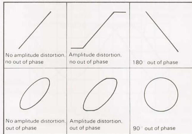
Fig. 17. Typical X-Y Phase Measurement Displays.
