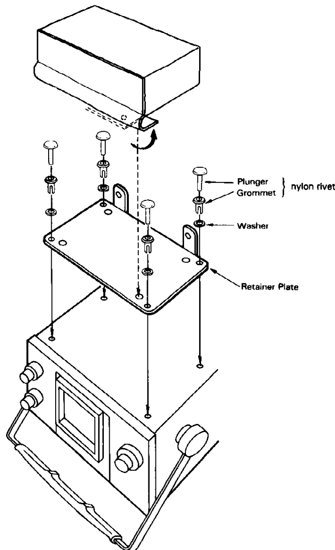
Fig. 40 Installation of LC-150 Probe Pouch.
