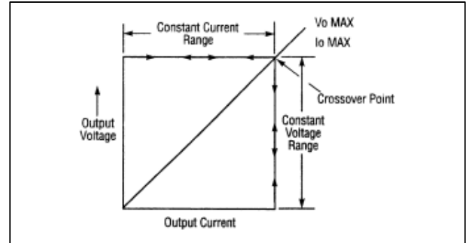
Figure 7. Constant Voltage/Constant Current Characteristic.
