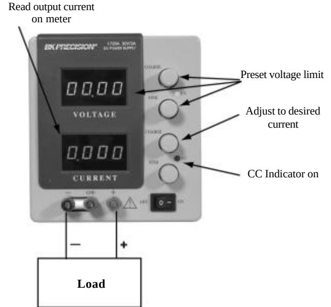
Figure 6. Typical Constant Current Operation.
