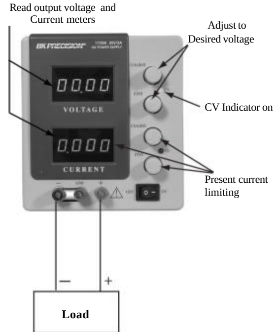
Figure 4. Typical Constant Voltage Operation.
