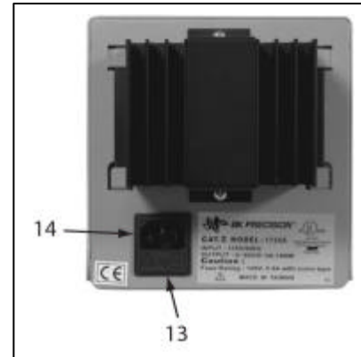
Figura 2. Panel trasero
