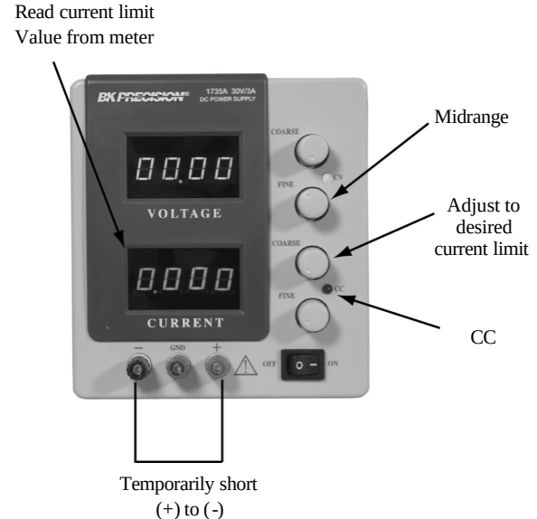
Figure 5. Setting Current Limit.
