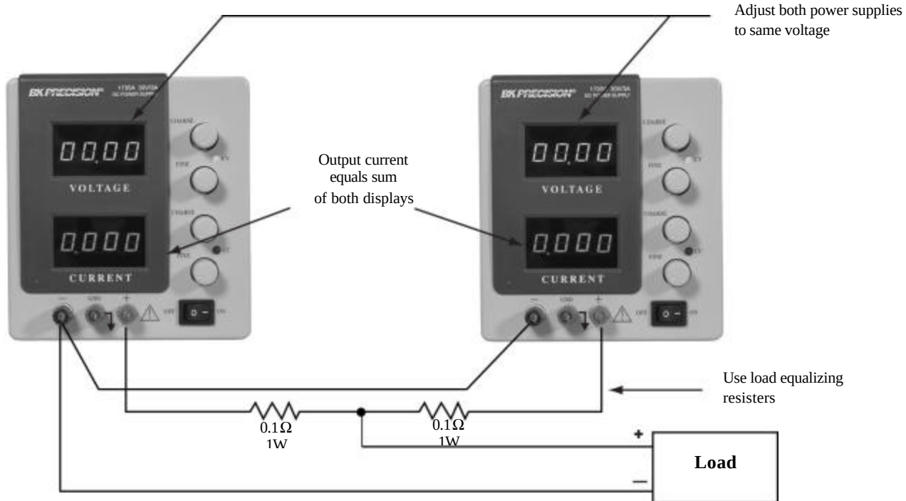
Figure 9. Connecting Two Power Supplies in Parallel.
