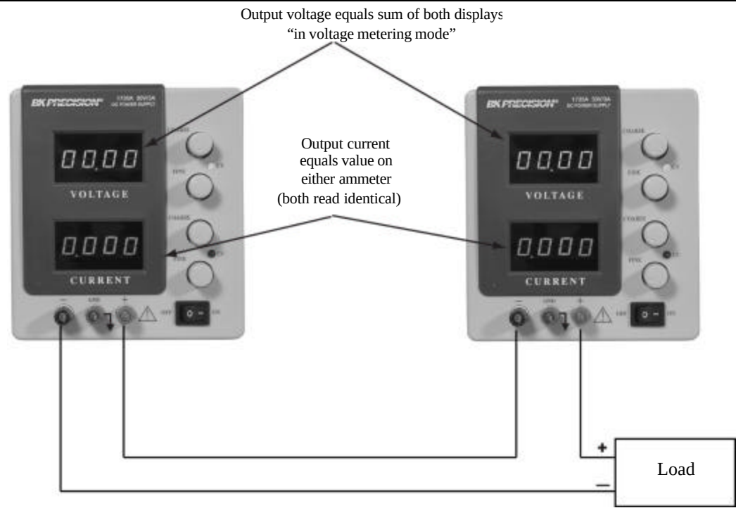
Figure 8. Connecting Two Power Supplies in Series.
