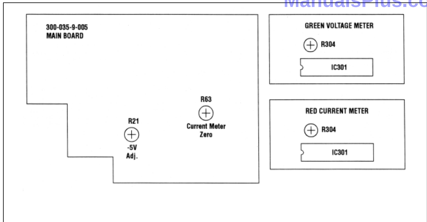
Figure 11. Location of Adjustments.
