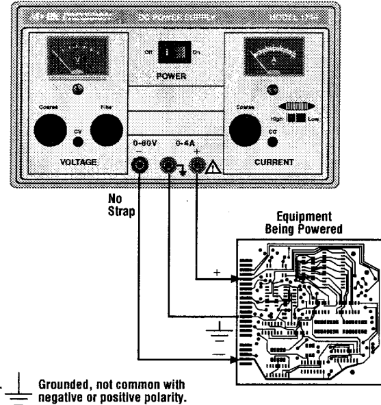
Figure 3 (C and D). Grounding Possibilities.
