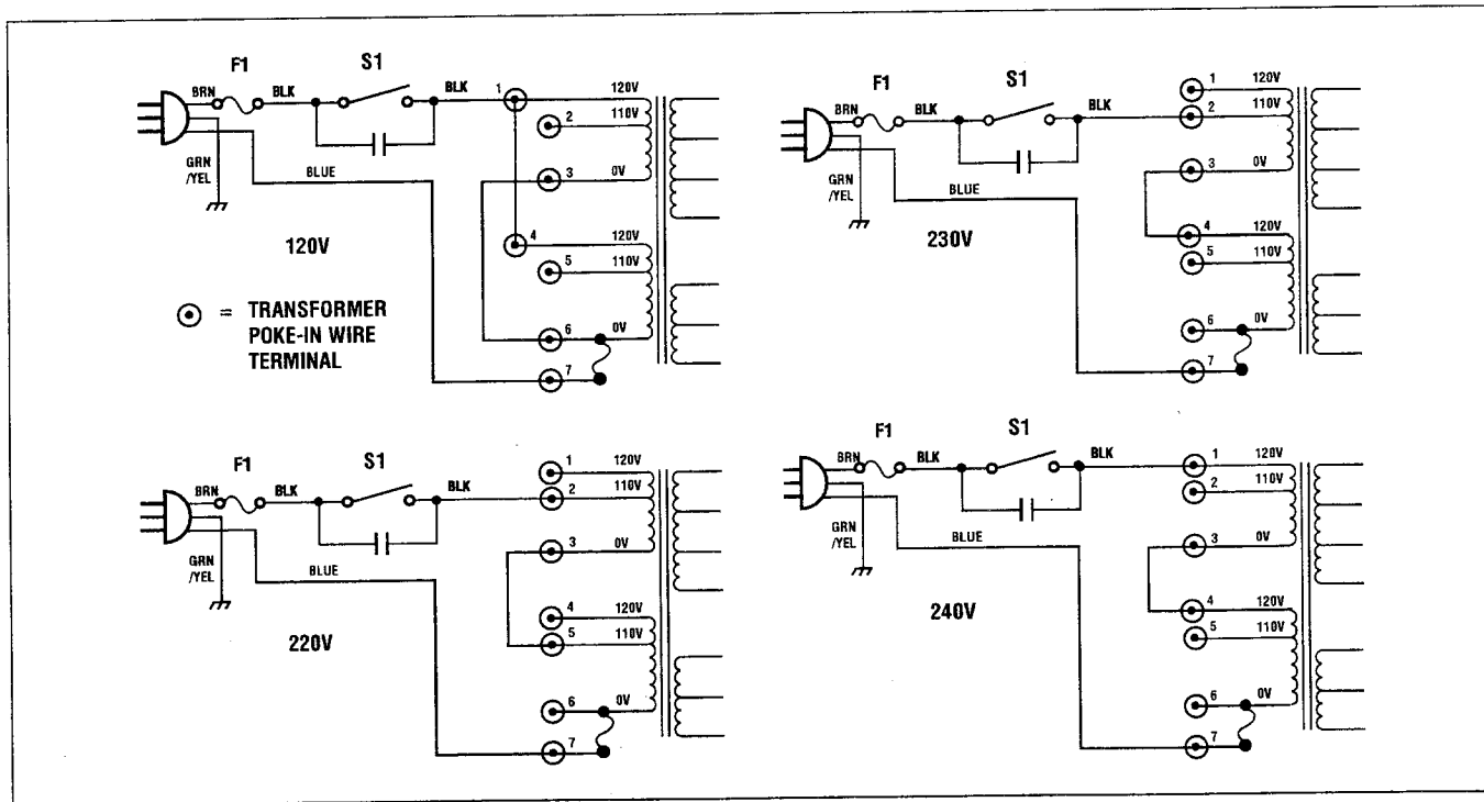
Figure 10. Line Voltage Conversion, International Units
