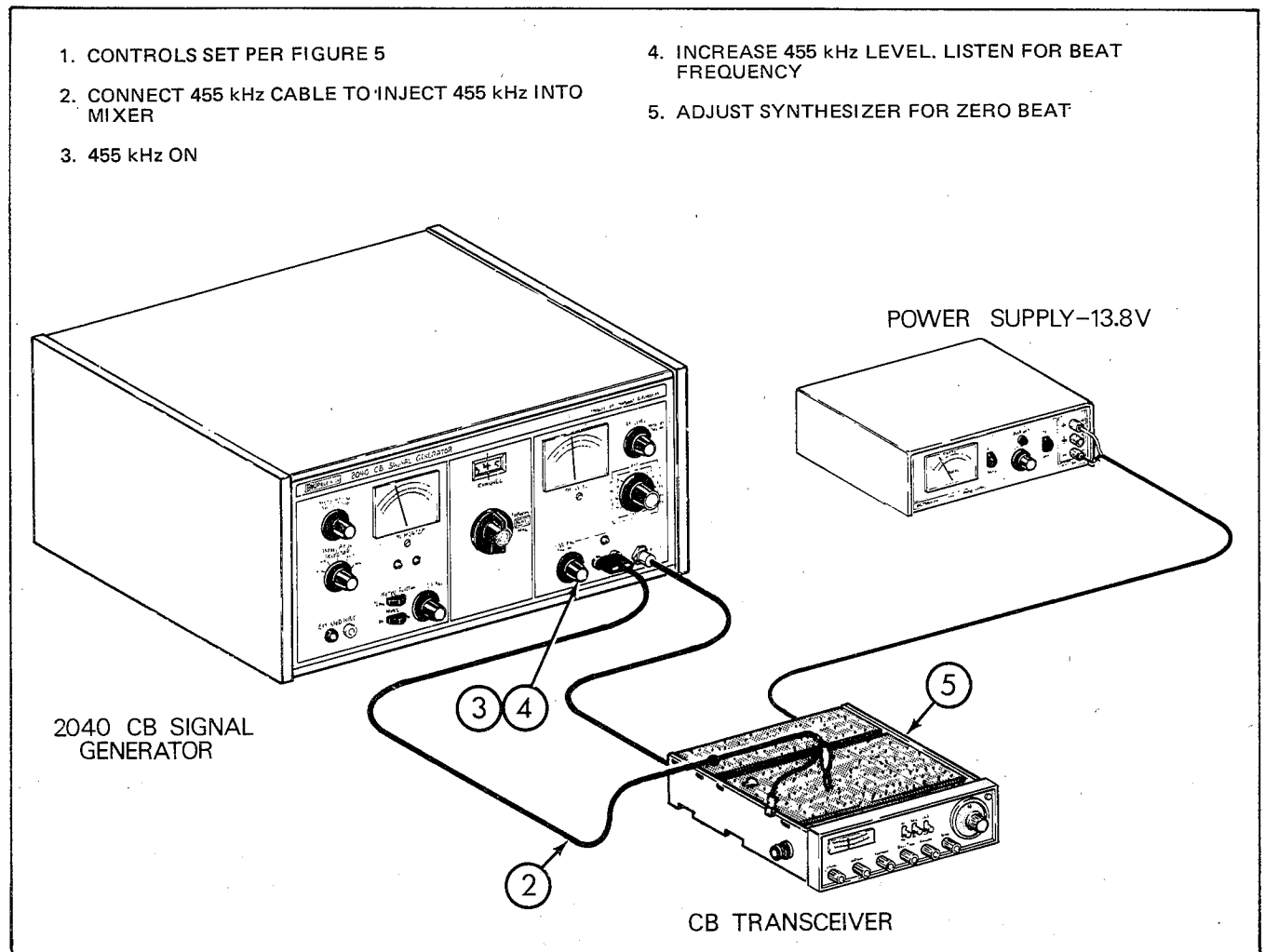
Fig. 18. Synthesizer frequency check and adjustment.
