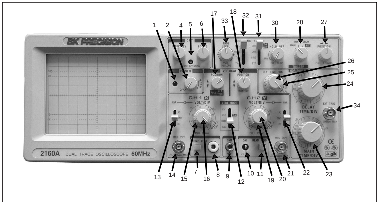
Fig. 1. Model 2160A Controls and Indicators.
