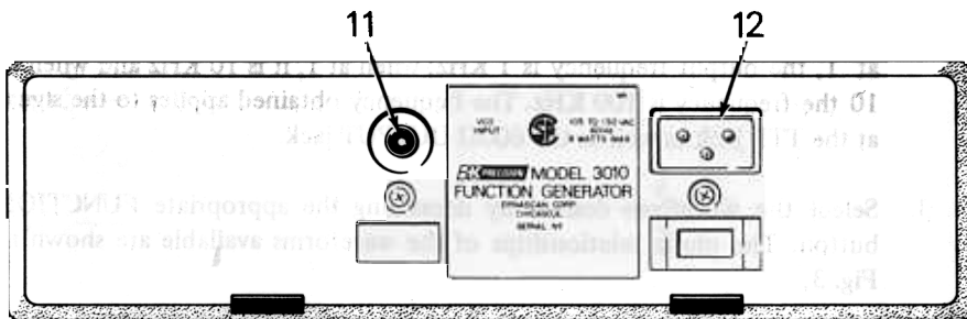
Fig. 2. Rear panel.
