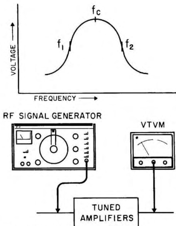
Figure 8. Making Gain Measurements
