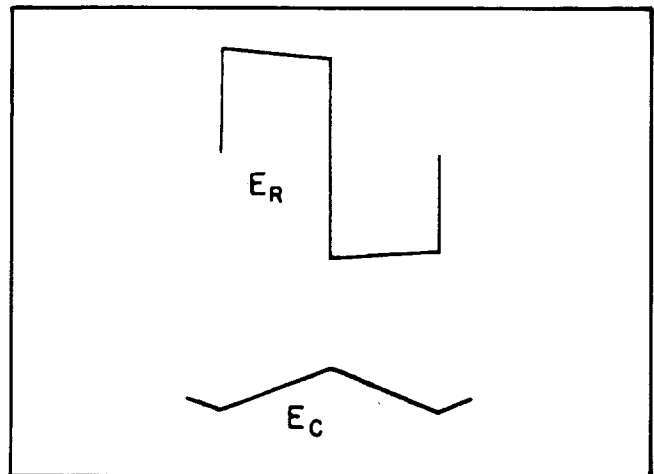
Figure 18. Waveforms Across R and C Using a High Frequency Square Wave
