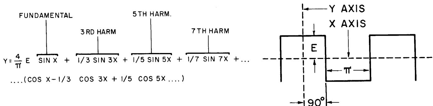
Figure 9. Fourier's Mathematical Description of a Square Wave.
