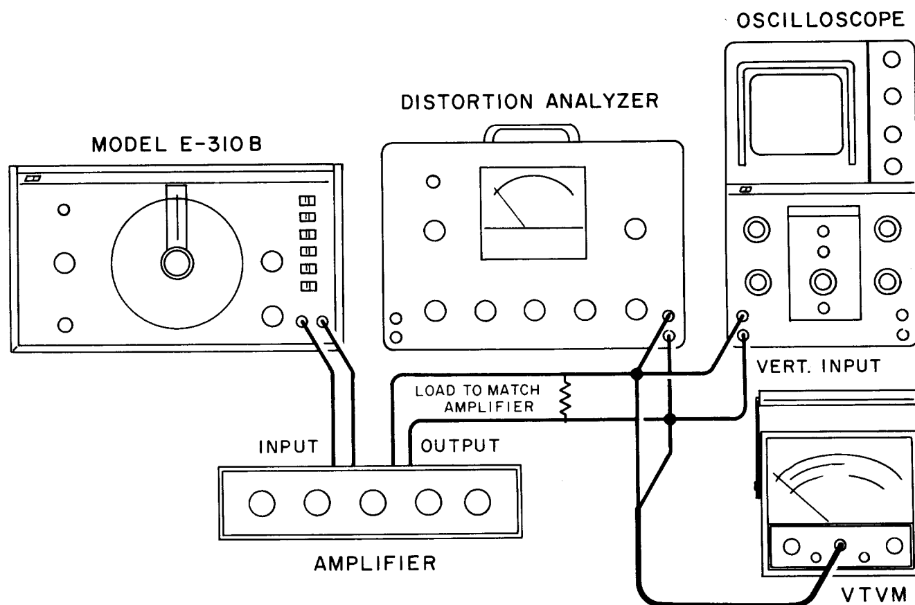
Figure 6. Typical Setup for Audio Amplifier Frequency Response and Distortion Measurements.
