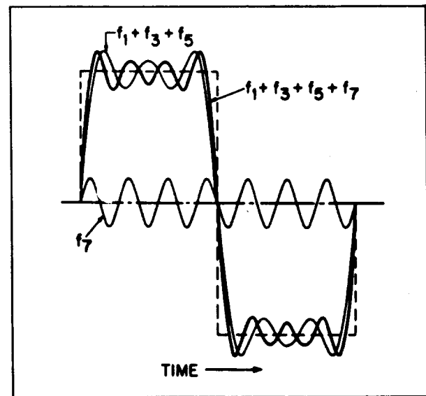
Figure 12. Loss of High Frequency Components of a Square Wave
