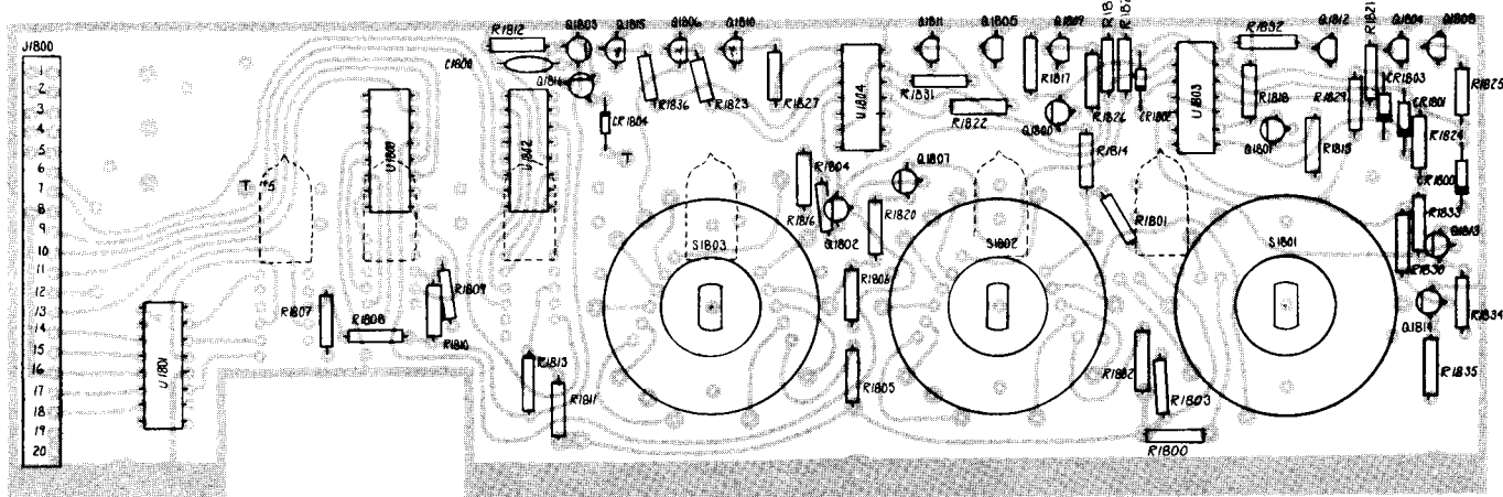
Figure 5-26. Display (A18)
