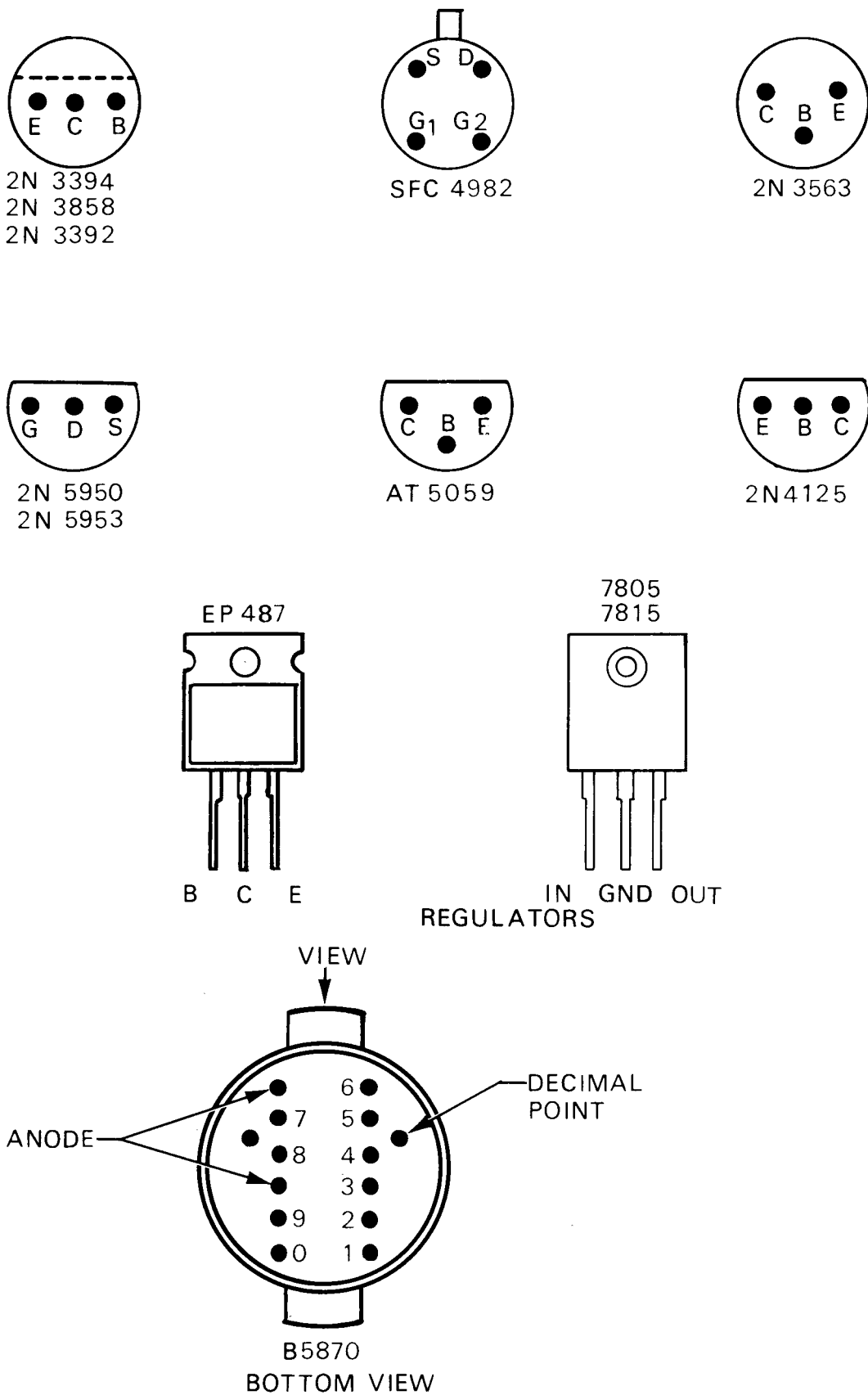
Figure 5-37. Component Lead Identification
