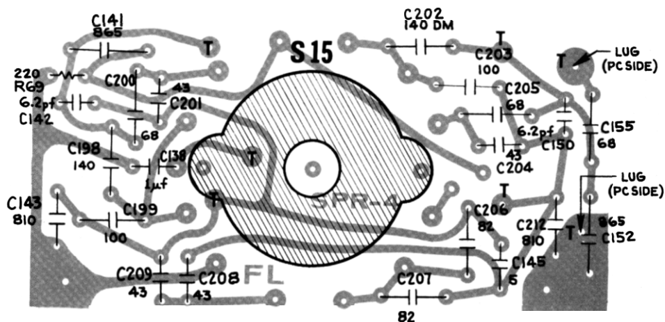
50 kHz FILTER CIRCUIT BOARD
