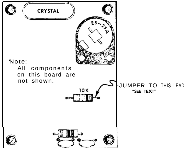
RY-4 CALIBRATION CONNECTION TO SPR-4
