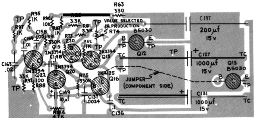
AUDIO AMPLIFIER CIRCUIT BOARD
