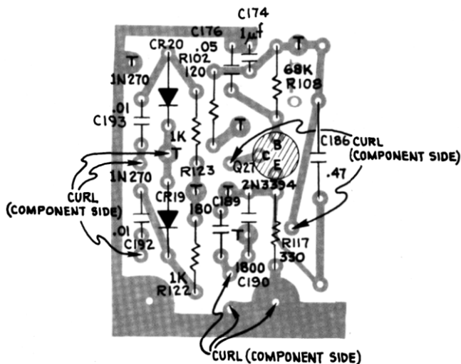
BFO CIRCUIT BOARD
