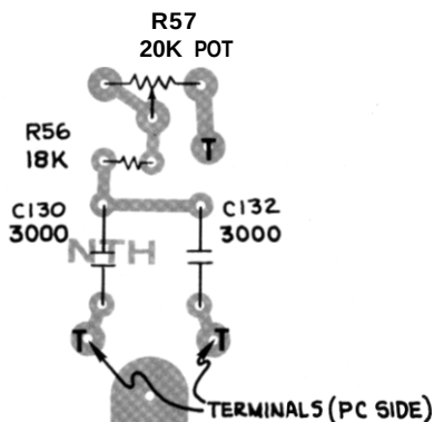
NOTCH FILTER CIRCUIT BOARD
