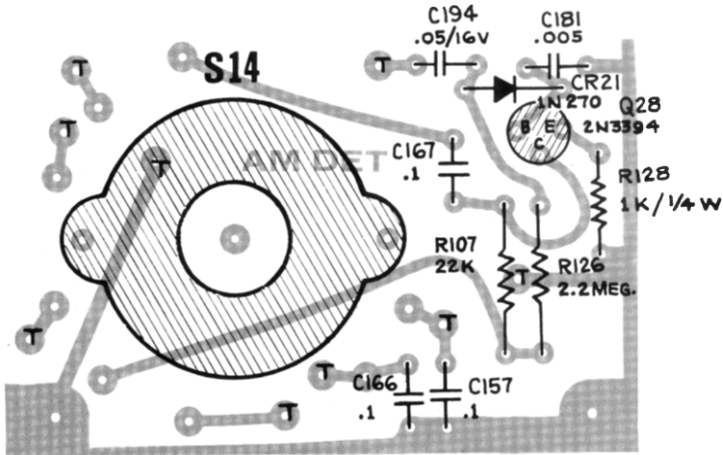
AM DETECTOR CIRCUIT BOARD
