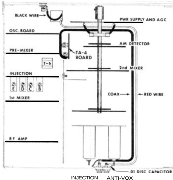
INJECTION ANTI-VOX TA4 CIRCUIT BOARD INSTALLATION DIAGRAM (c) R.L. DRAKE VIRTUAL MUSEUM
