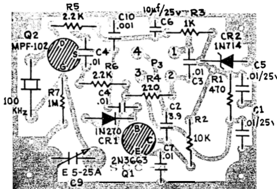
SCC-4 CIRCUIT BOARD
