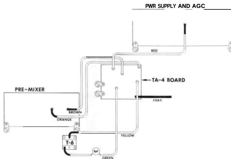
TA-4 PICTORAL WIRING DIAGRAM (c) R.L. DRAKE VIRTUAL MUSEUM
