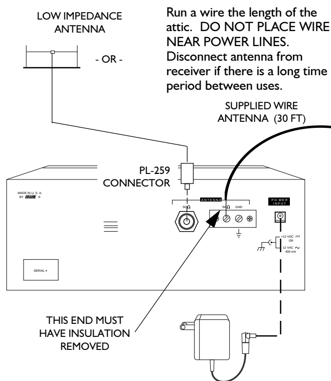
FIGURE 2 - BASIC ANTENNA CONNECTIONS
