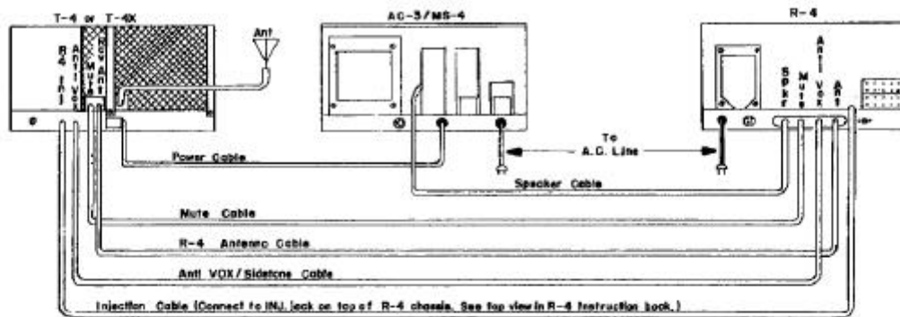
FIG. 1 CONNECTING THE T-4 OR T-4X TO THE R-4 RECEIVER, AC-3 POWER SUPPLY, AND MS-4 SPEAKER.
