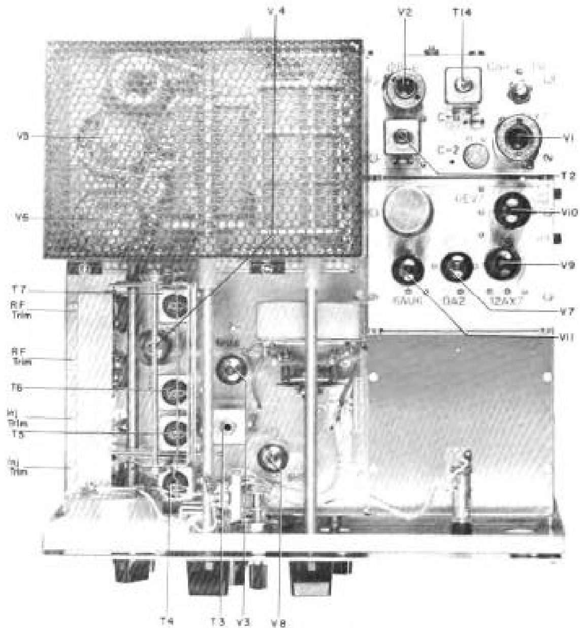
FIGURE 12 TOP VIEW T-4
