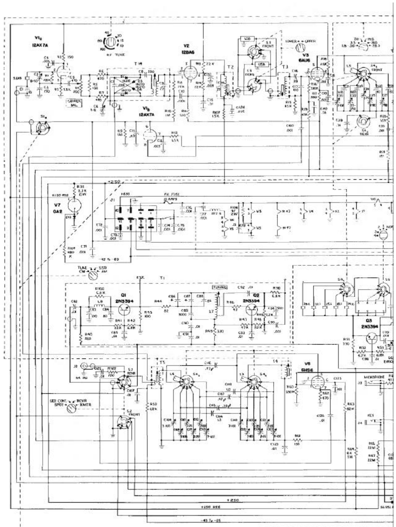
SCHEMATIC DIAGRAM MODEL T
