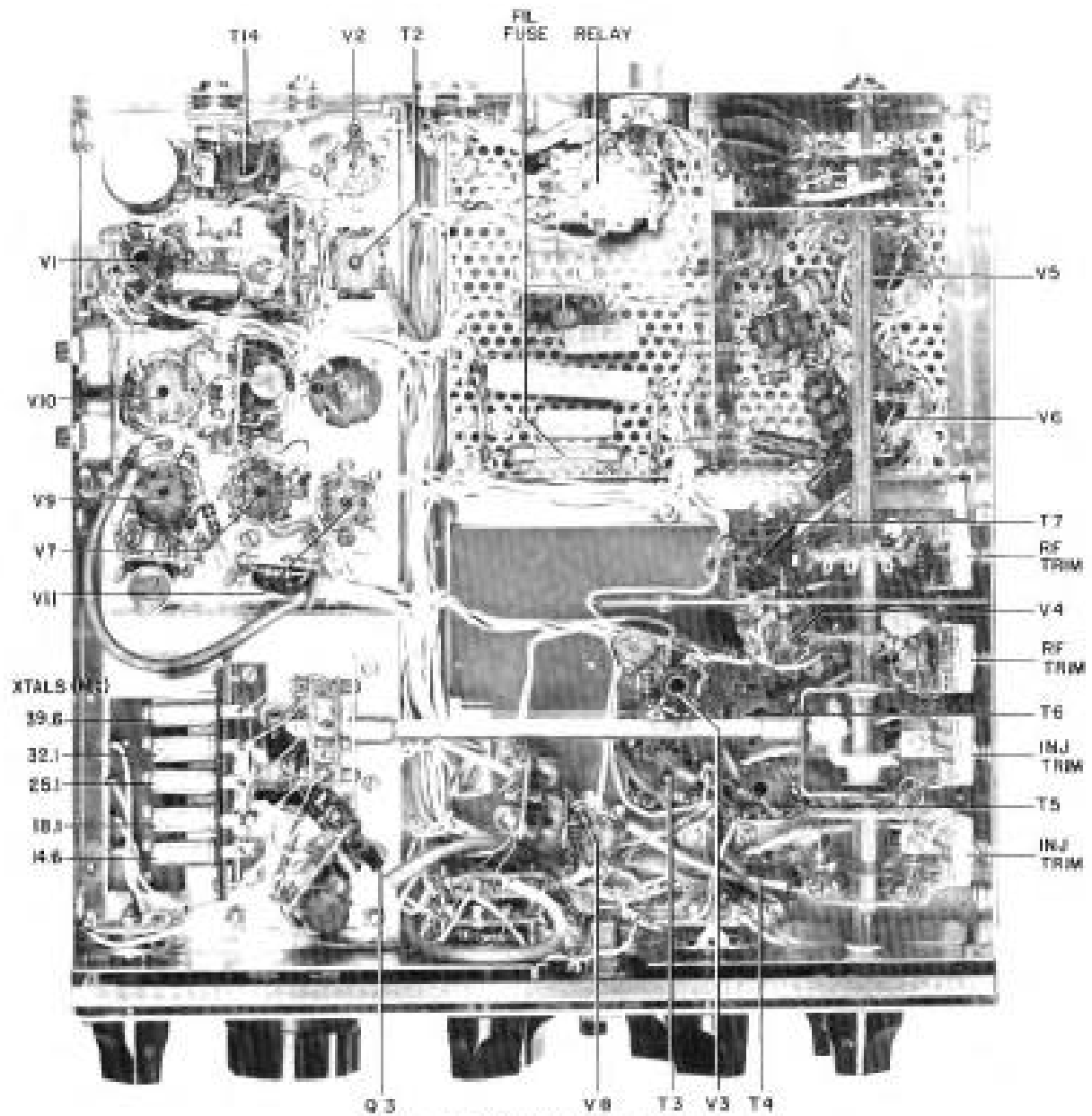
FIGURE 15 BOTTOM VIEW T-4X
