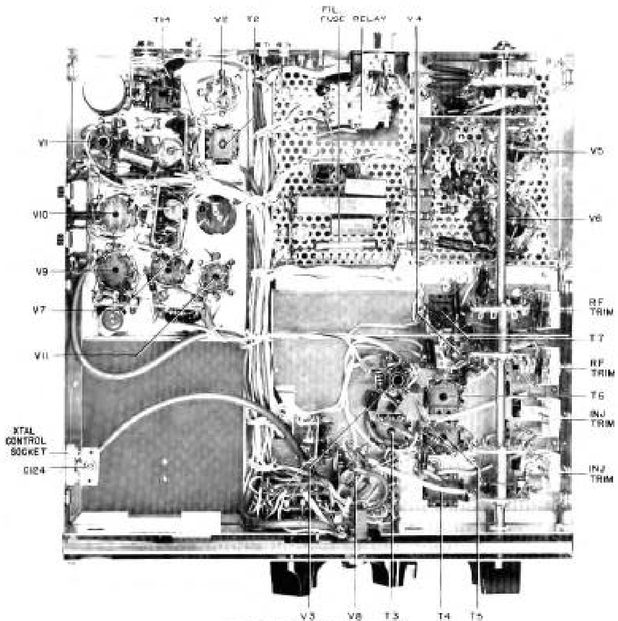
FIGURE 13. BOTTOM VIEW T-4
