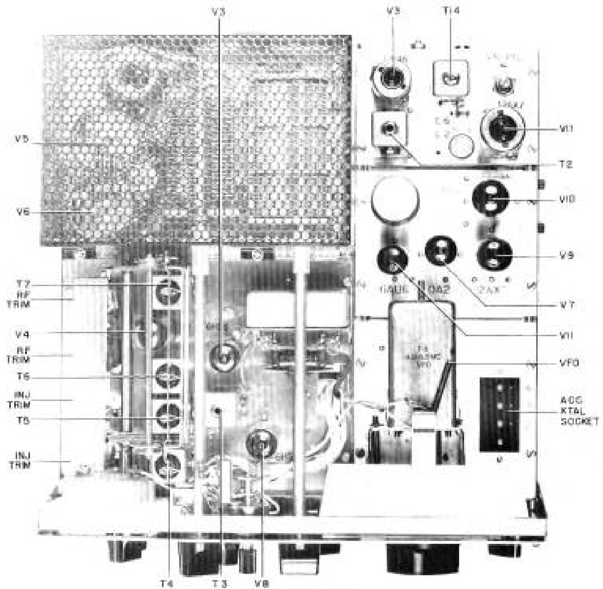
FIGURE 14 TOP VIEW T-4X
