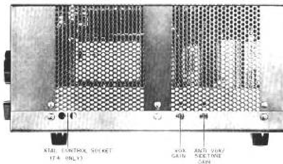
FIGURE 5 SIDE VIEW
