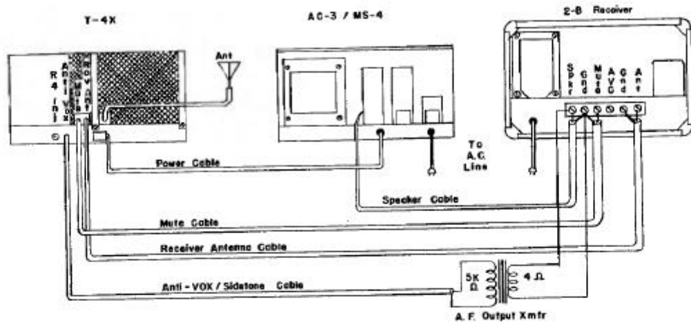
FIG. 3 CONNECTING THE T-4X TO A RECEIVER OTHER THAN THE R-4
