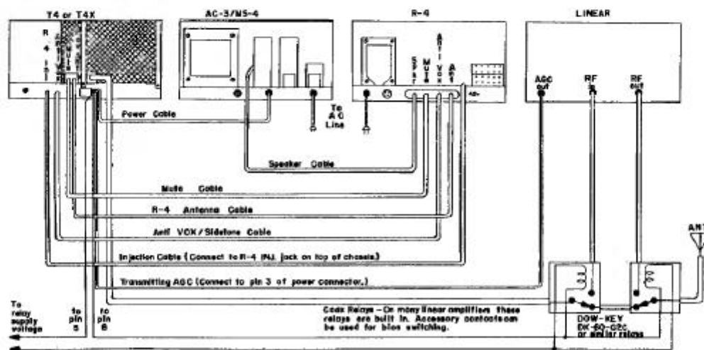
FIG. 2 CONNECTING THE T-4 OR T-4X TO A LINEAR AMPLIFIER
