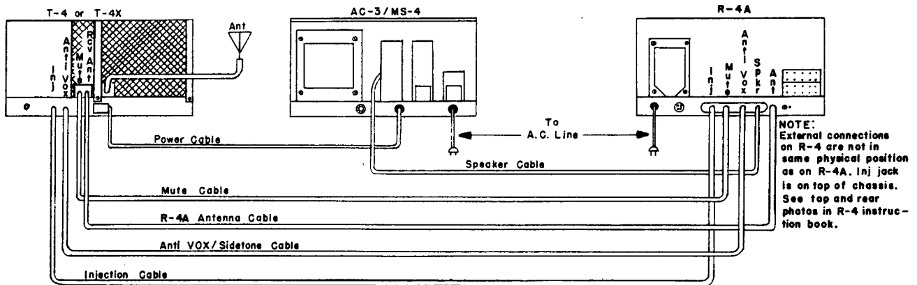
FIG. 1 CONNECTING THE T-4 OR T-4X TO THE R-4A RECEIVER, AC-3 POWER SUPPLY, AND MS-4 SPEAKER.
