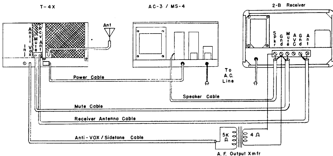
FIG. 3 CONNECTING THE T-4X TO A RECEIVER OTHER THAN THE R-4 OR R-4A
