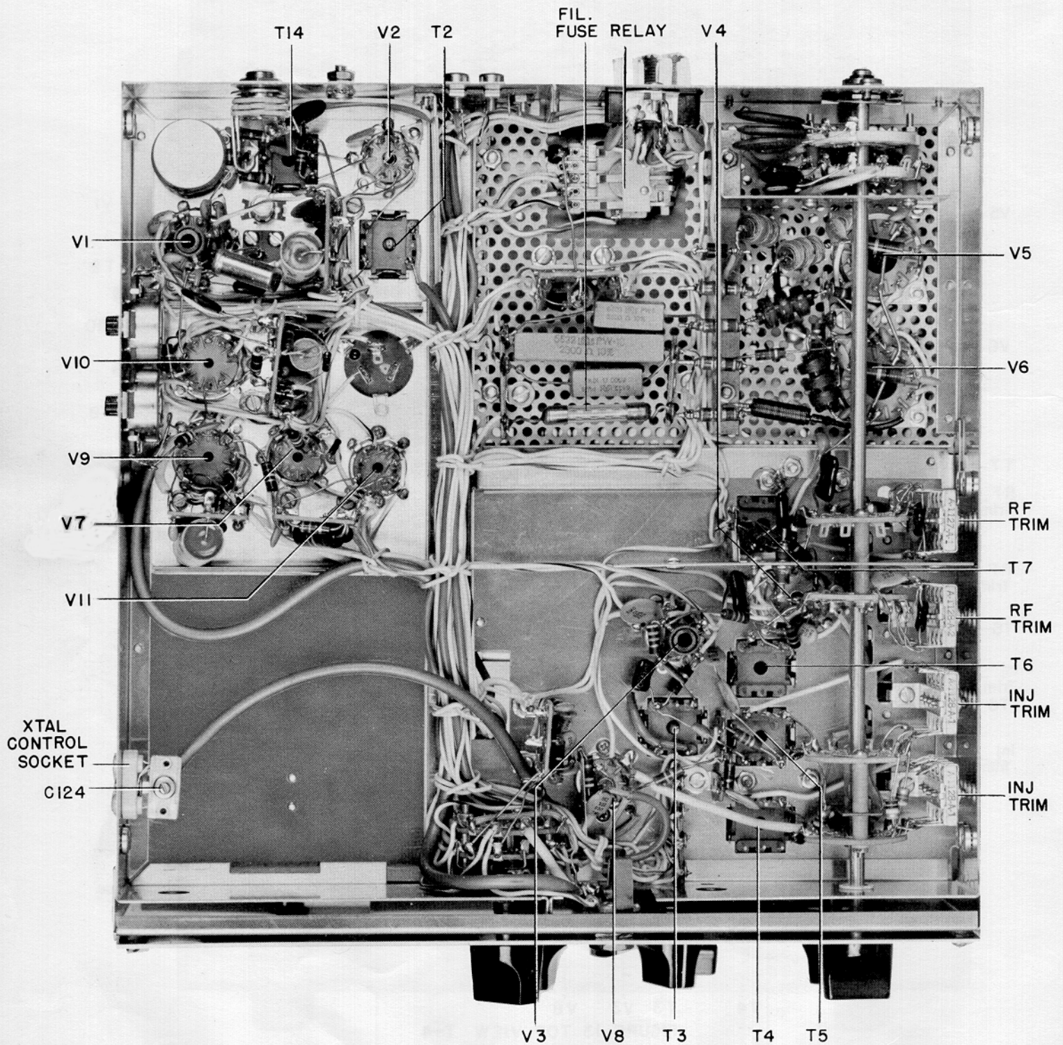
FIGURE 14 BOTTOM VIEW T-4
