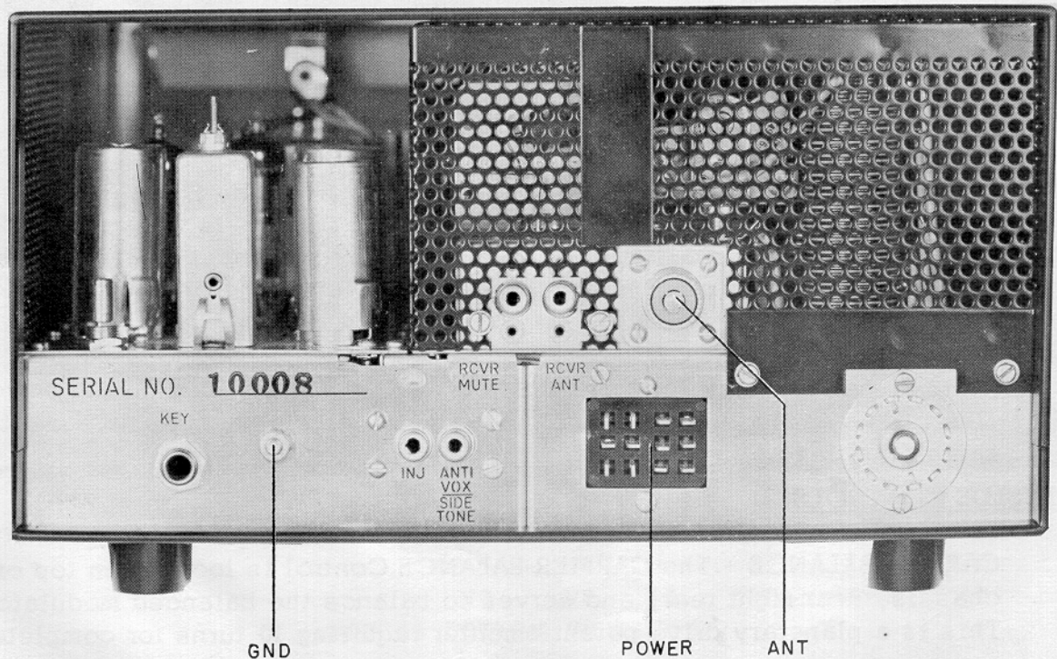
FIGURE 6 REAR VIEW
