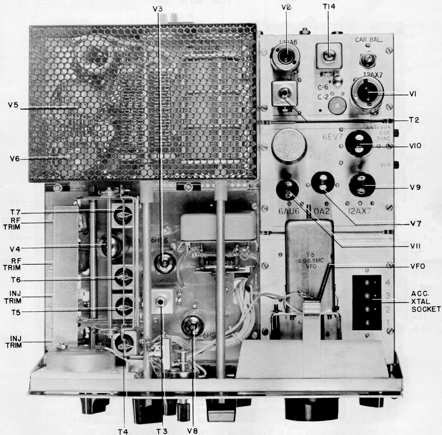
FIGURE 15 TOP VIEW T-4X
