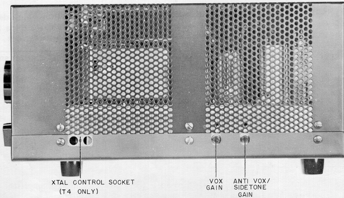
FIGURE 5 SIDE VIEW
