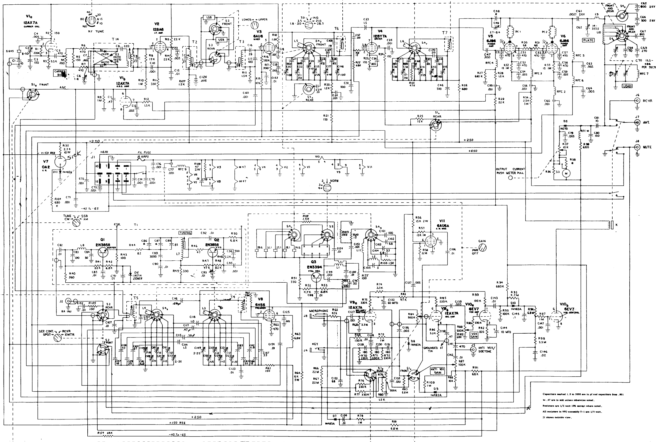
SCHEMATIC DIAGRAM MODEL T-4X TRANSMITTER
