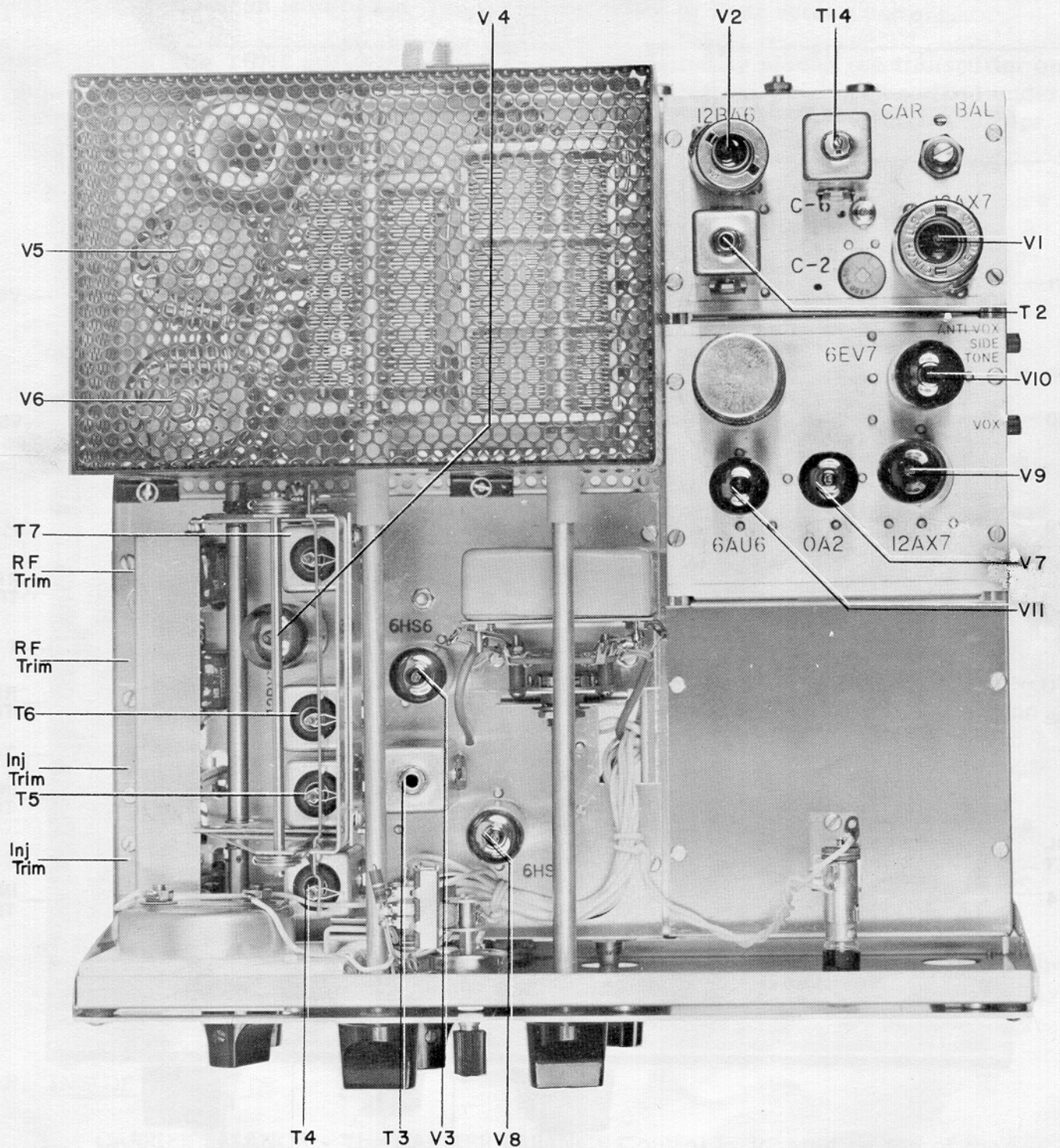
FIGURE 13 TOP VIEW T-4
