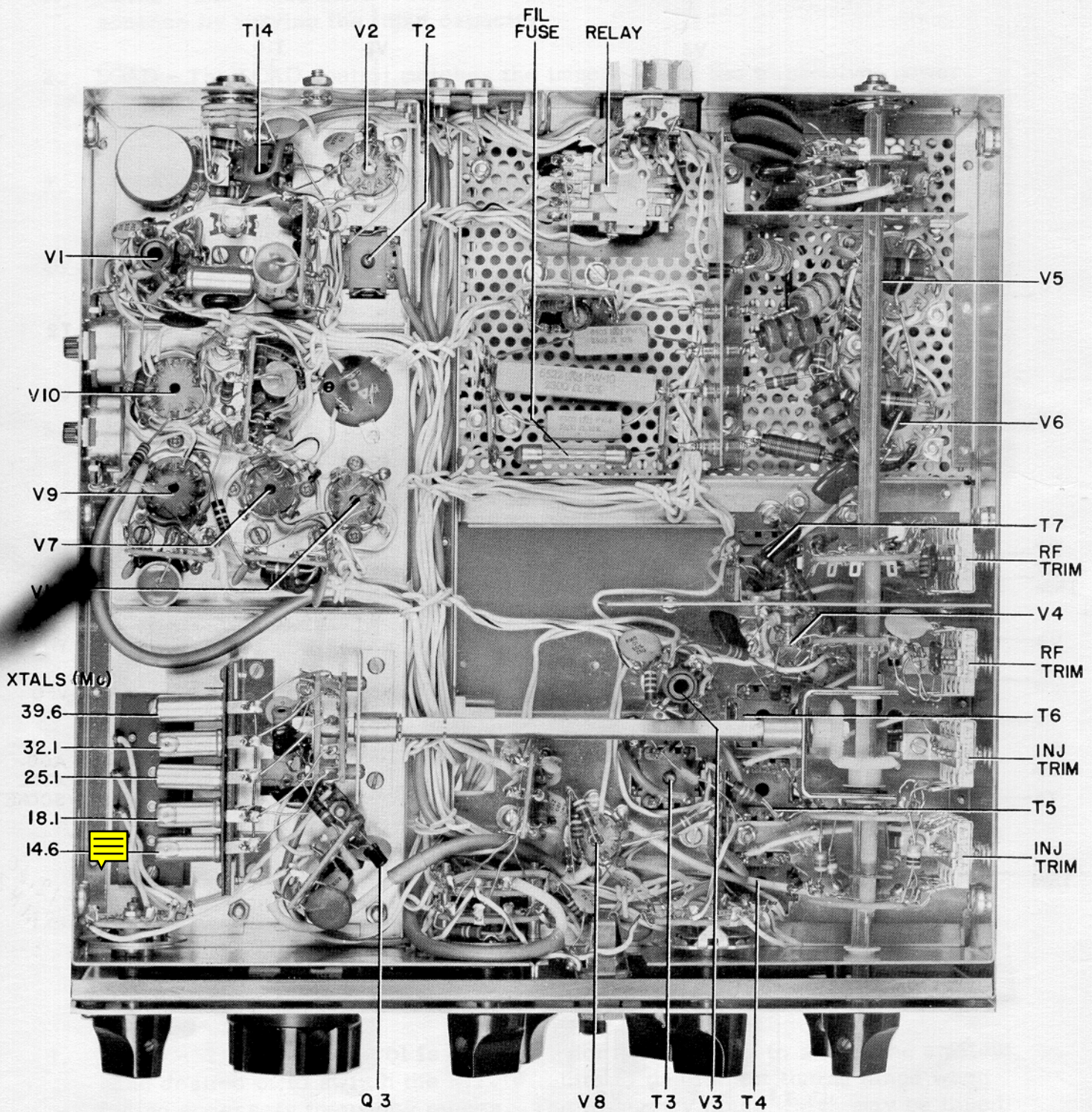
FIGURE 16 BOTTOM VIEW T-4X
