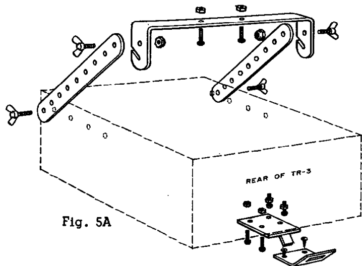
Fig. 5 MECHANICAL DETAILS OF MOBILE INSTALLATION USING MMK-3 MOBILE MOUNTING KIT
