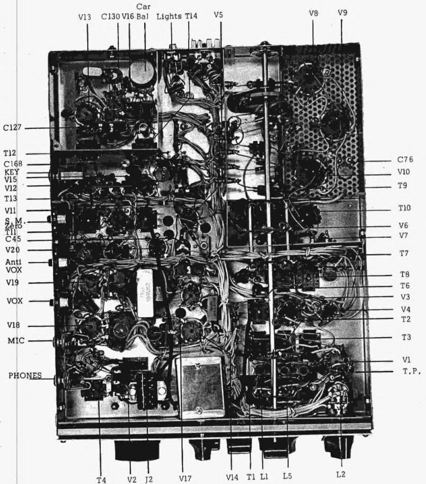
Figure 11 BOTTOM VIEW
