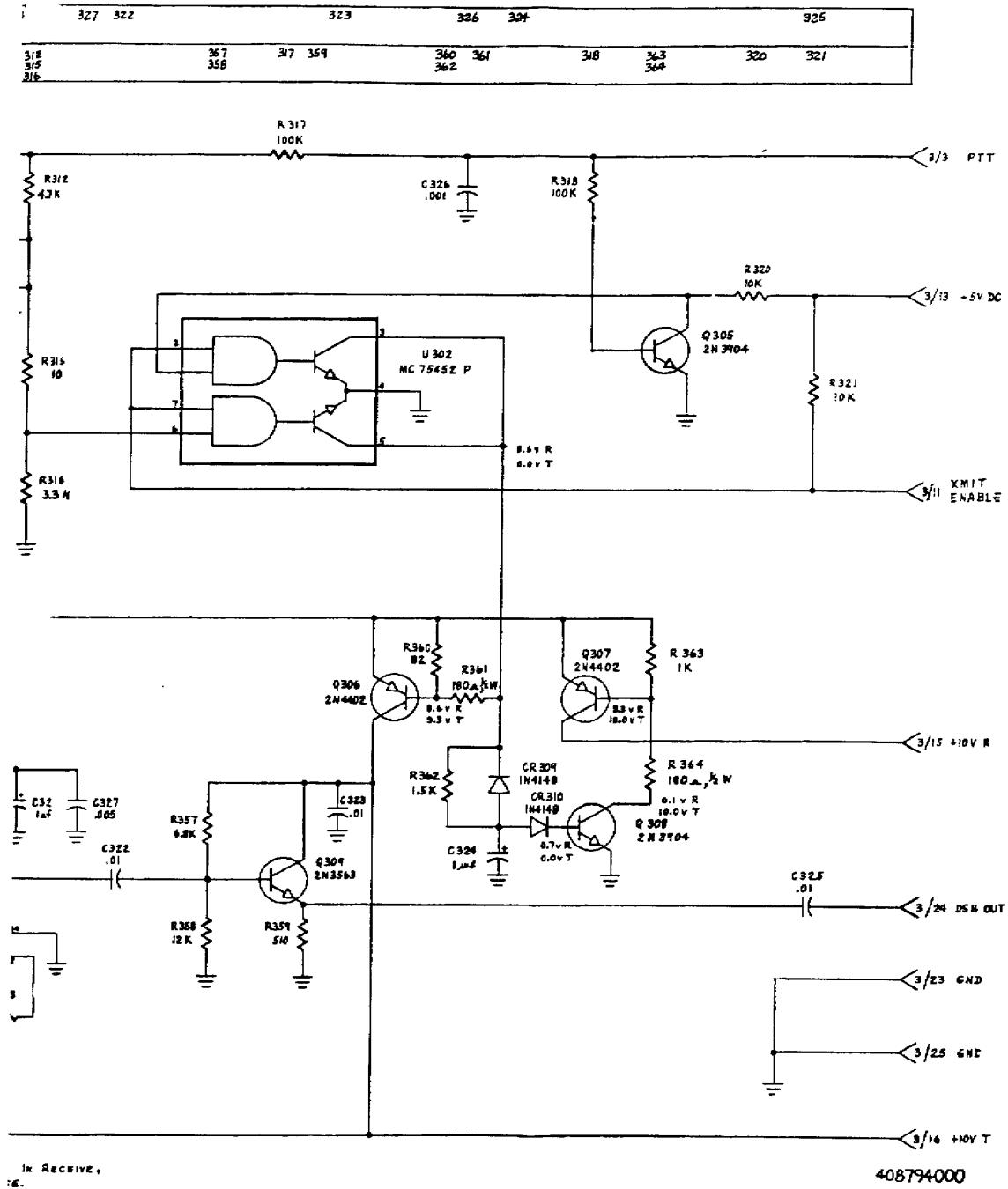
Fig. 2-8 Transmit Exciter Board Schematic
