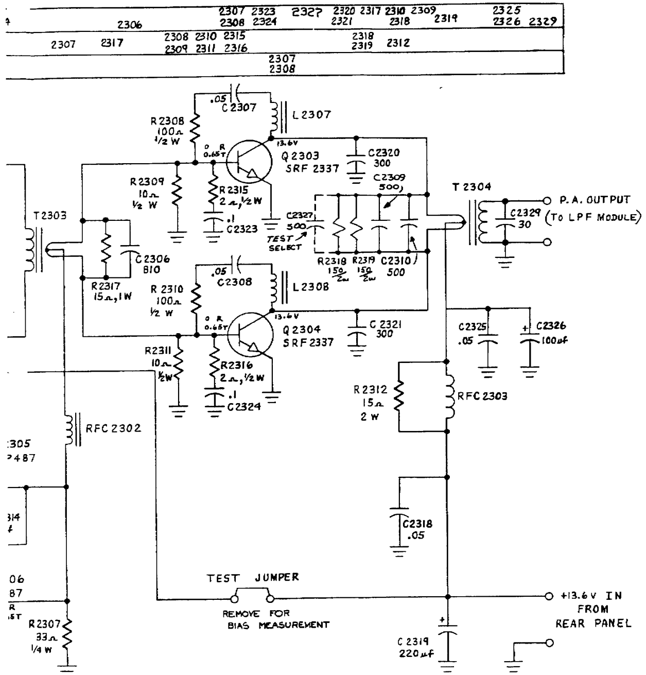
Fig. 2-42 Power Amplifier Schematic
