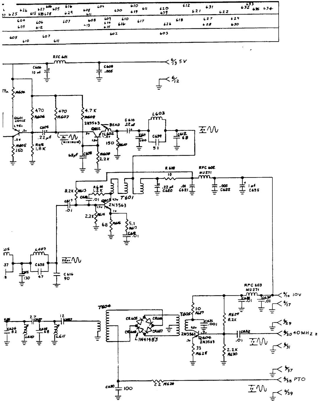
Fig. 2-14 Translator Board Schematic
