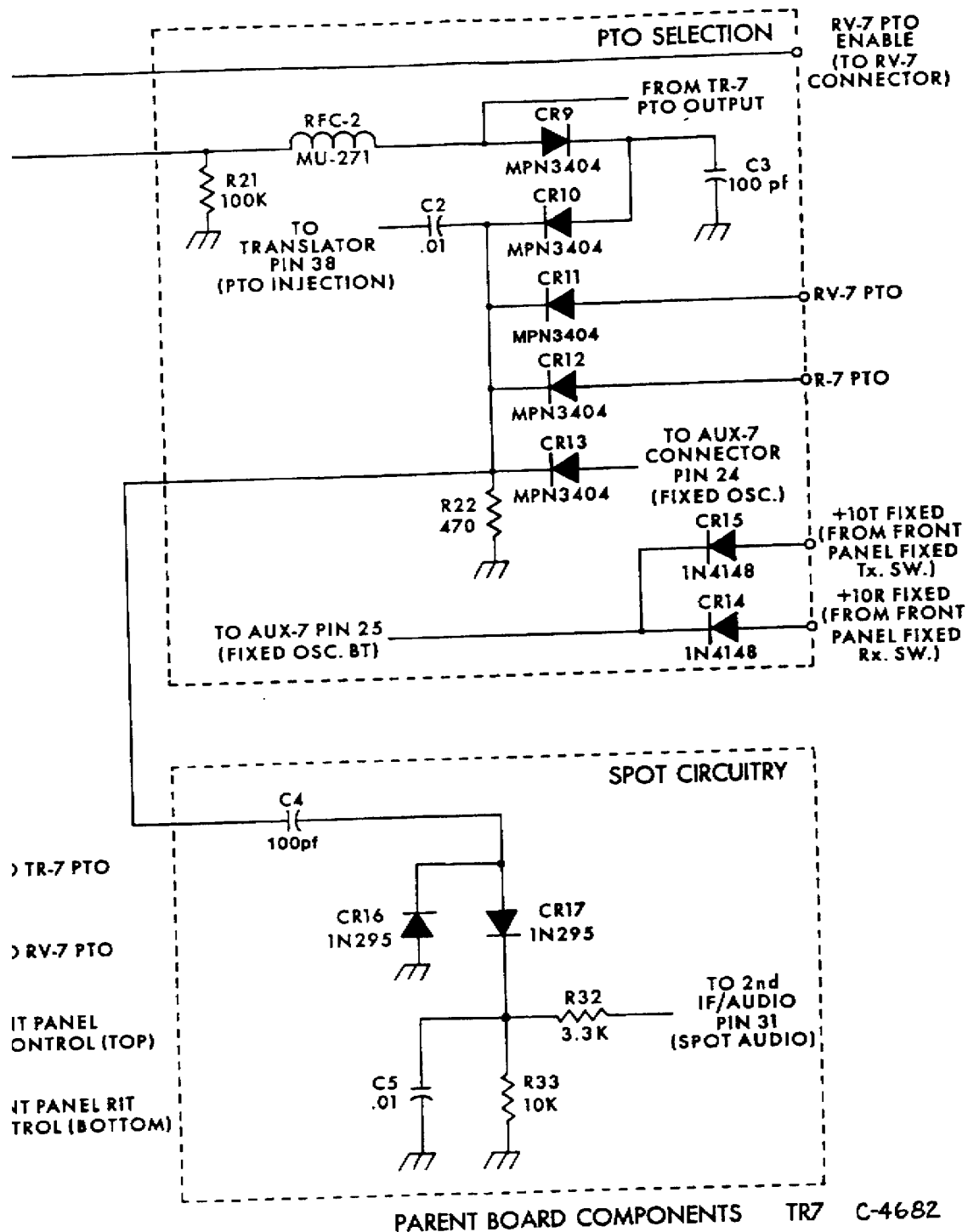
Fig. 2-4 RIT &amp; PTO Switching Schematic
