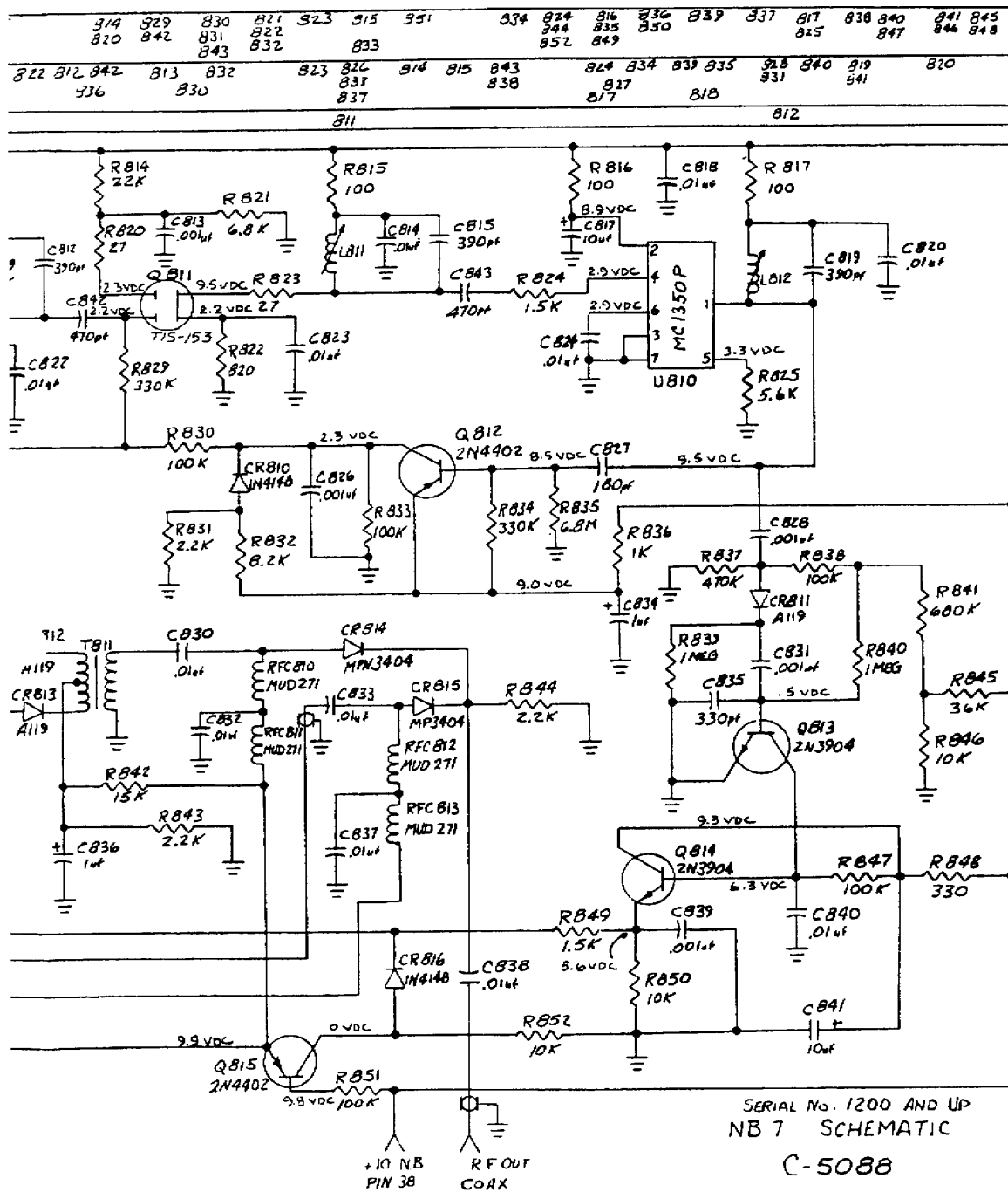
Fig. 4-9 NB-7 Board Schematic, Version 2
