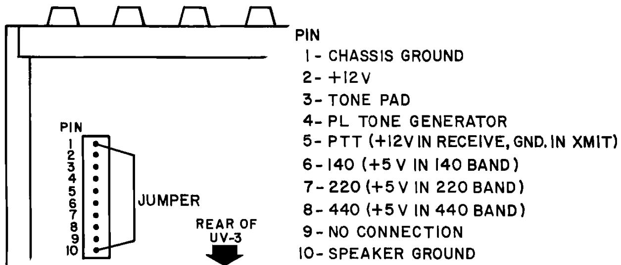
Figure 3-5. Auxiliary Connector
