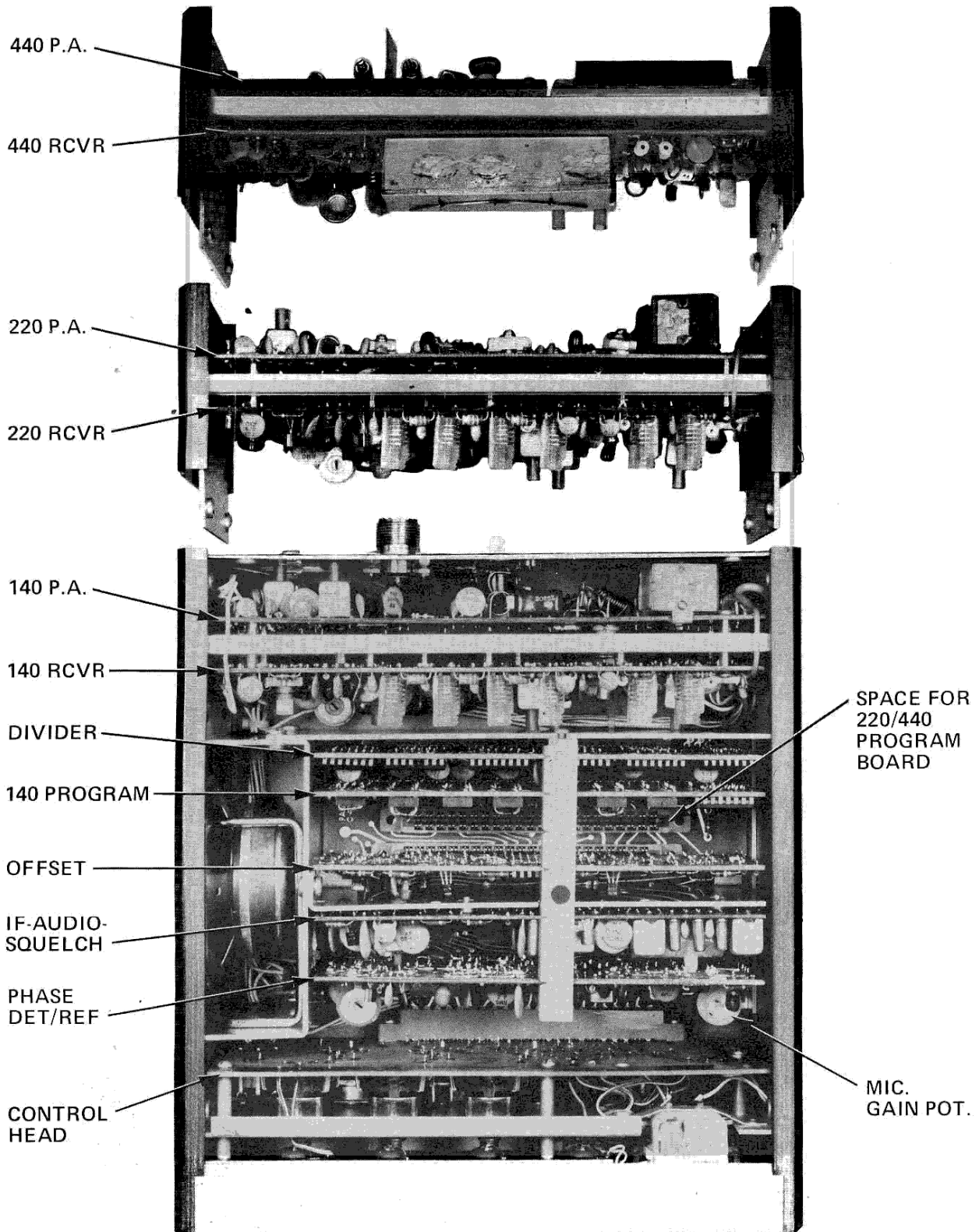
Figure 3-2. Board Locations
