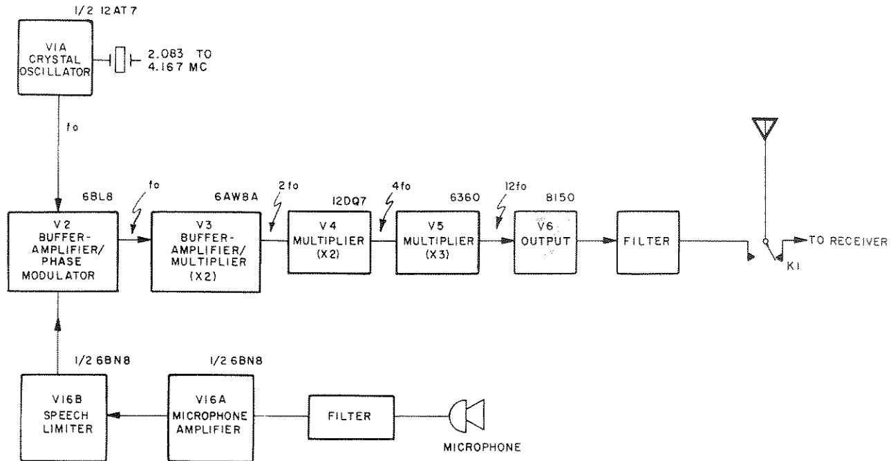
Figure 9. Transmitter Block Diagram
