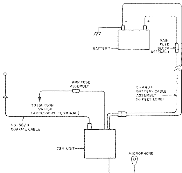
Figure 1. Front Mount Mobile Installation.
