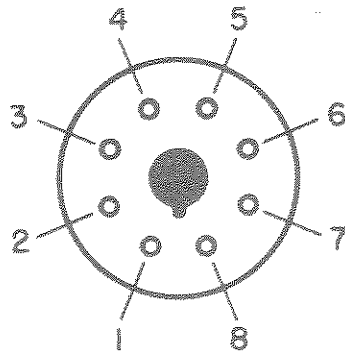
BOTTOM VIEW OF SOCKET
