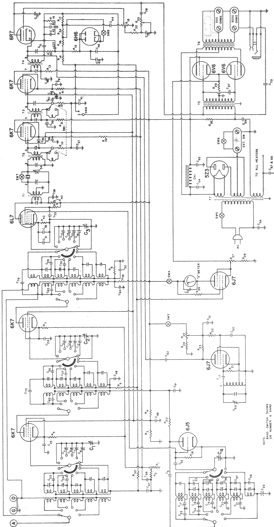
SCHEMATIC DIAGRAM — SUPER SKYRIDER — TYPE SX-17
