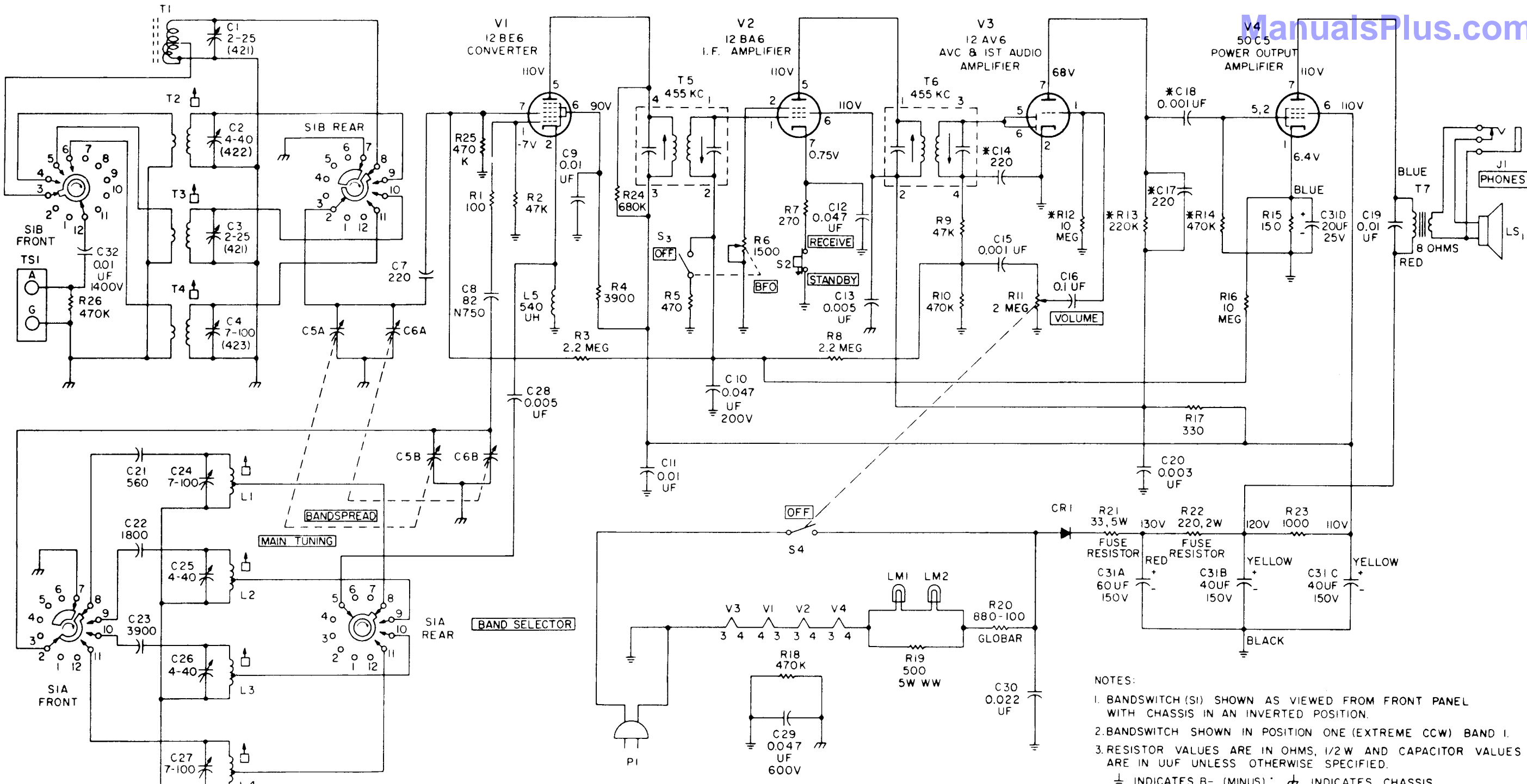
Hallicrafters S-120
