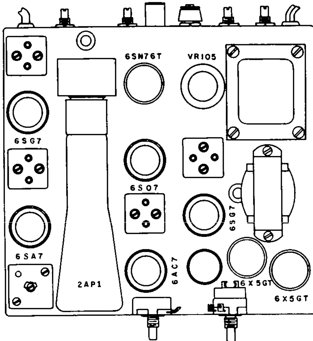
Figure 7. Skyrider Panoramic Model SP-44, top view showing tube locations.
