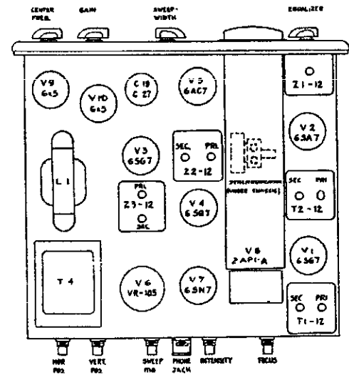
Fig. 3. Top View of Chassis.
