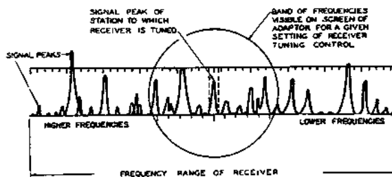
Figure 2. Portion of the Radio Spectrum.
