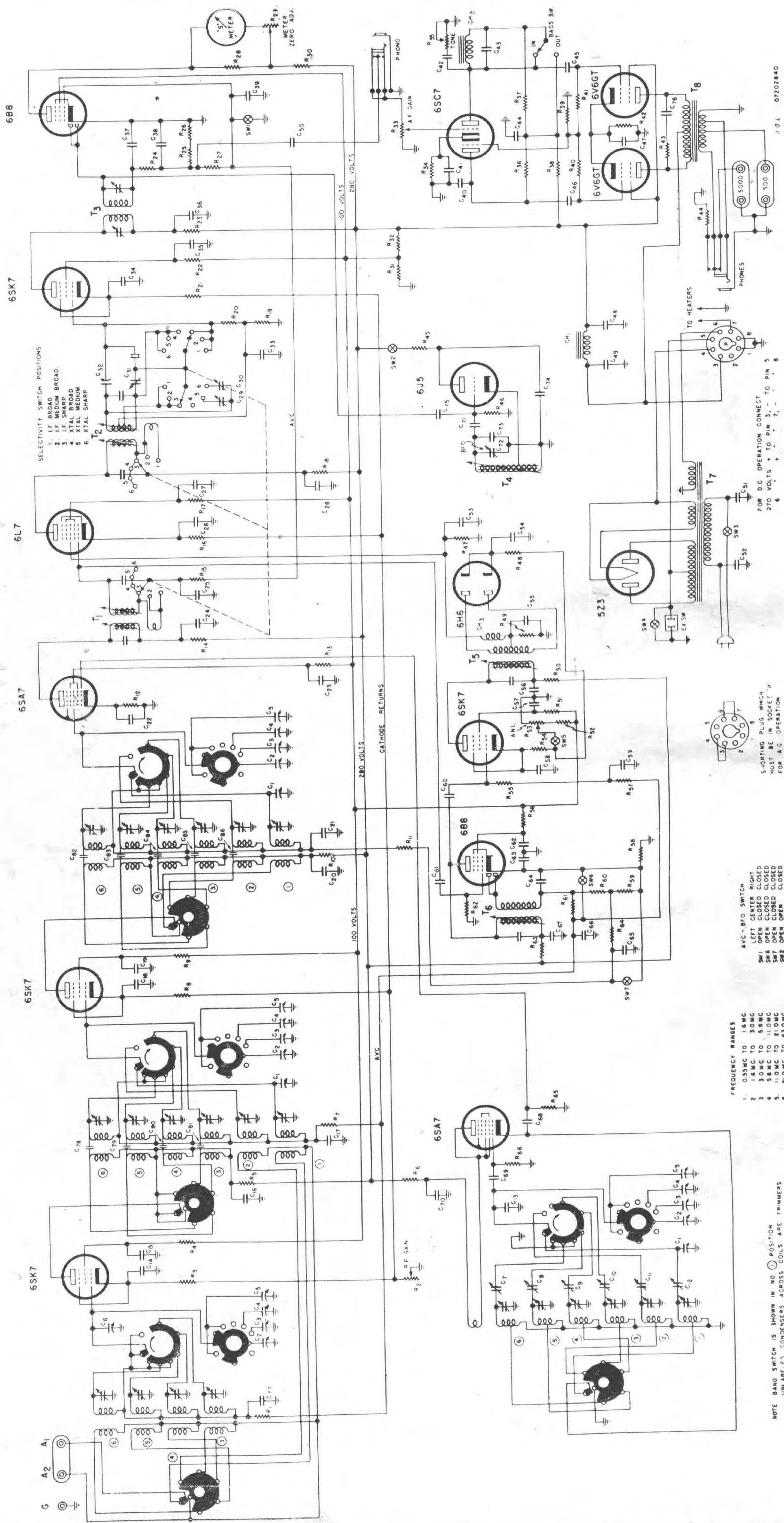
SCHEMATIC DIAGRAM - SUPER SKYRIDER - MODEL SX-23
