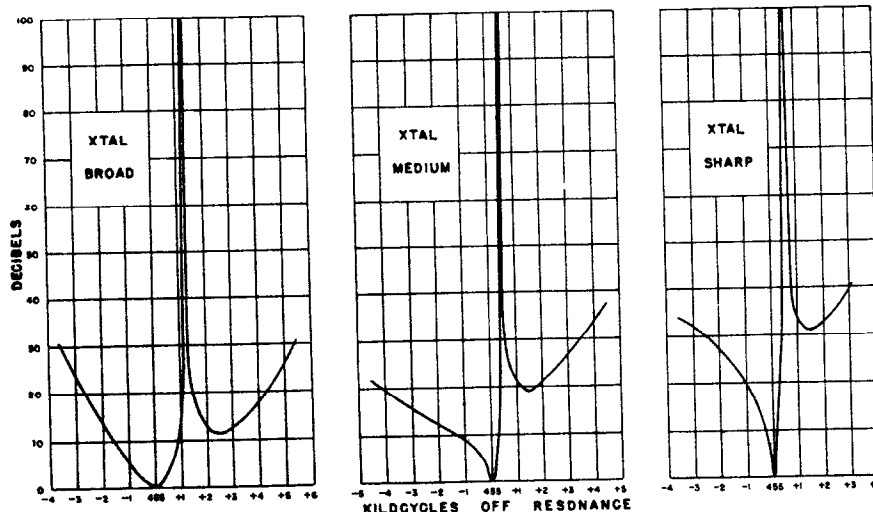
FIG. 4—CRYSTAL SELECTIVITY
