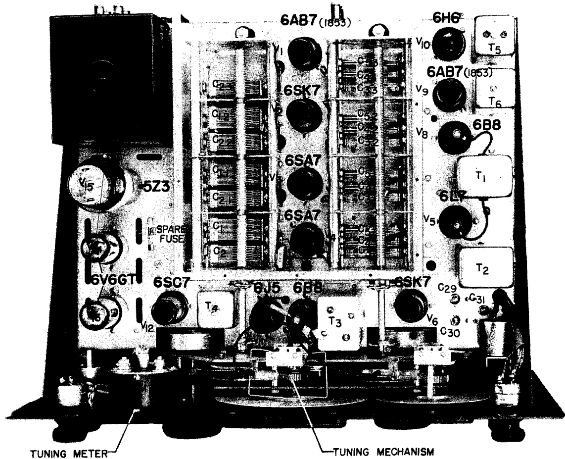
FIG. 9—SX28-A—REAR VIEW
