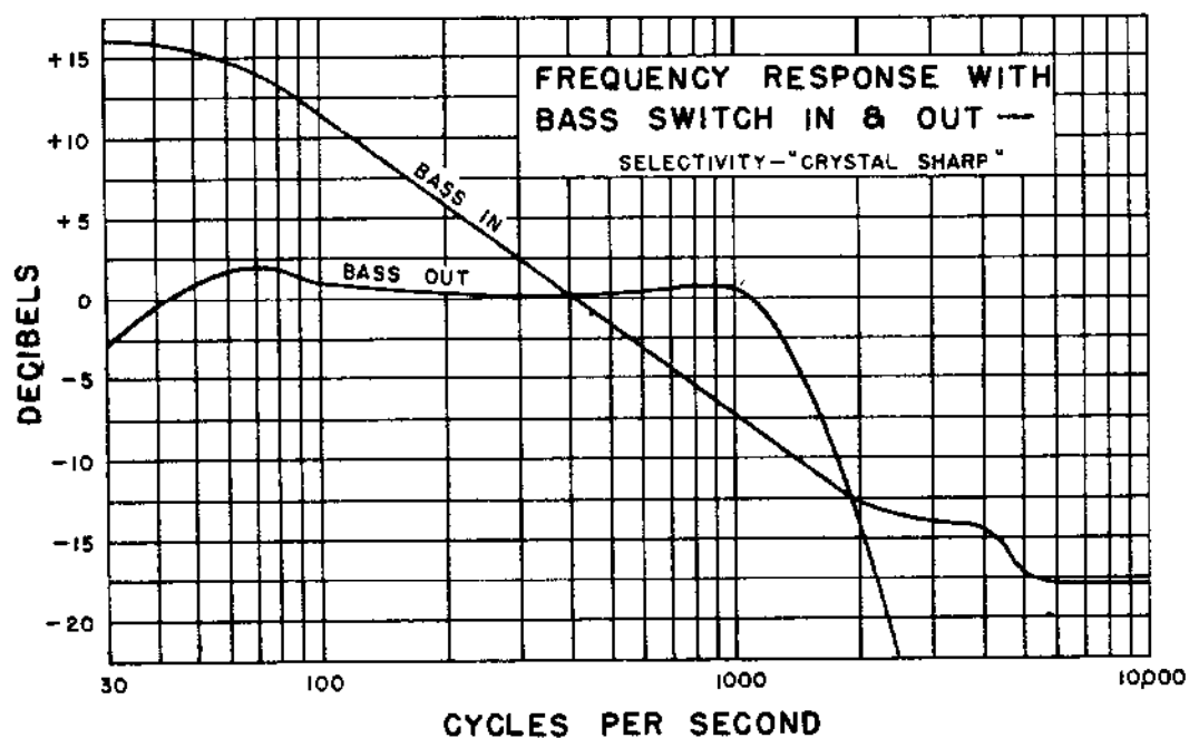
FIG. 11—AUDIO FILTER CURVE
