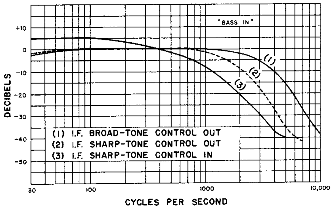
FIG. 10—AUDIO FIDELITY CURVE
