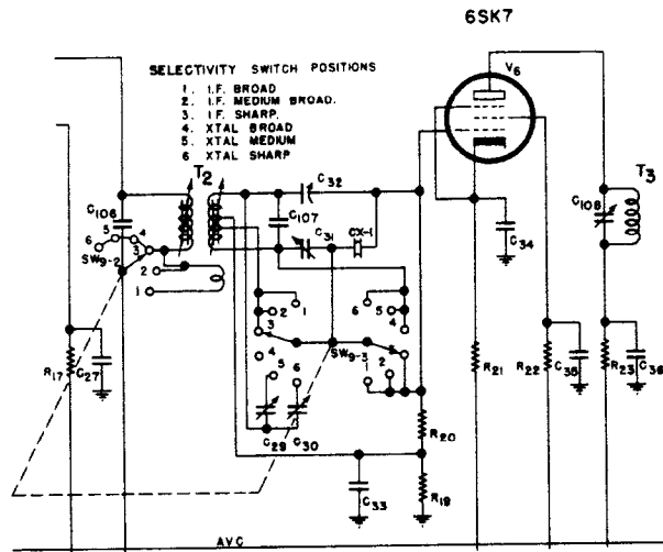
FIG. 2—CRYSTAL FILTER SCHEMATIC
