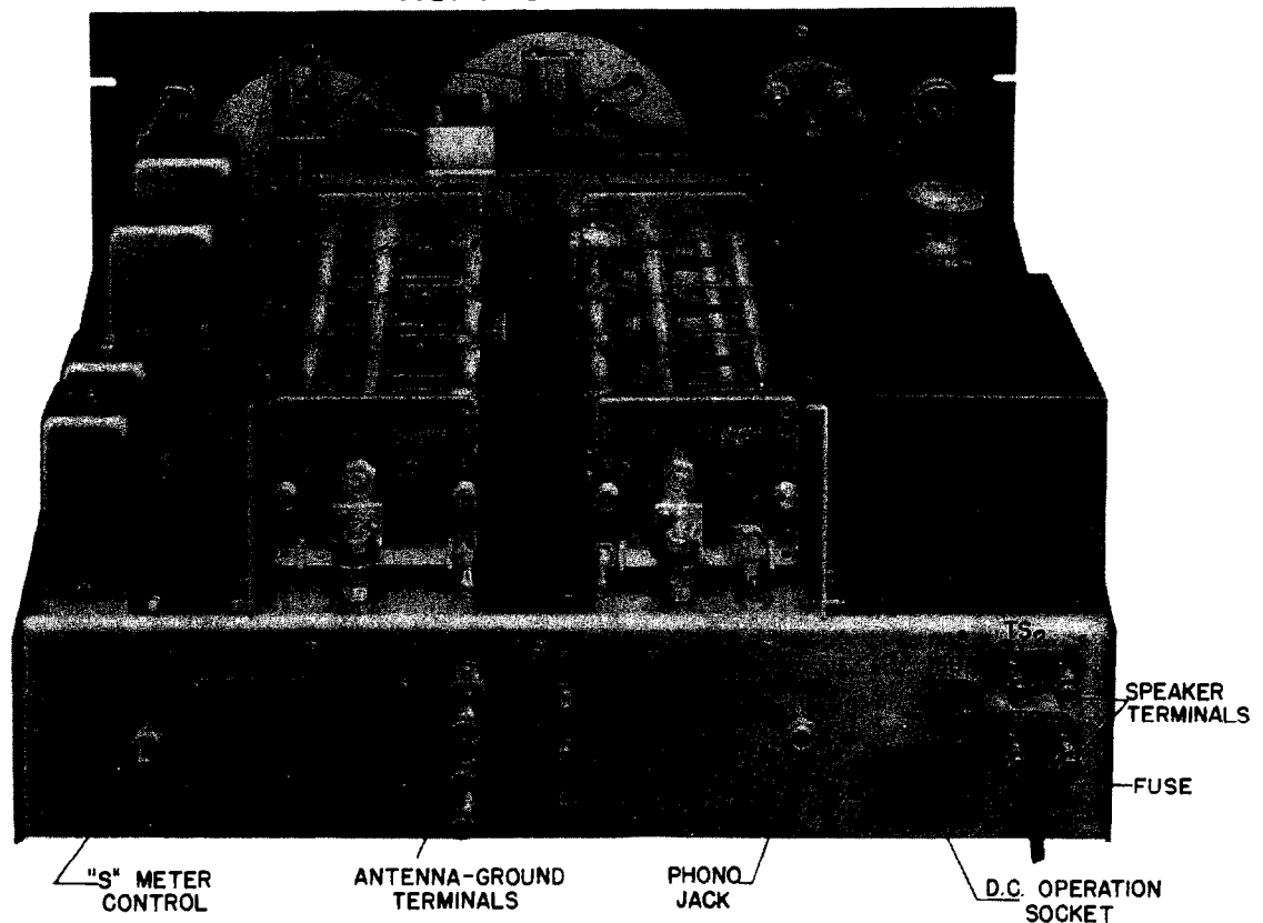
FIG. 9—SX28-A—REAR VIEW
