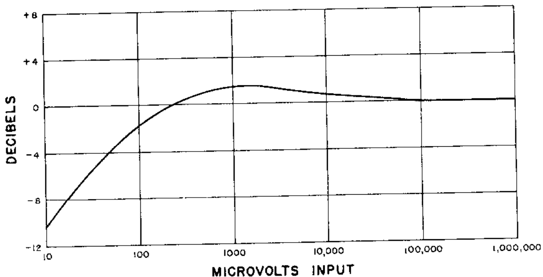
FIG. 7—A.V.C. CURVE—AT 3 MC.
