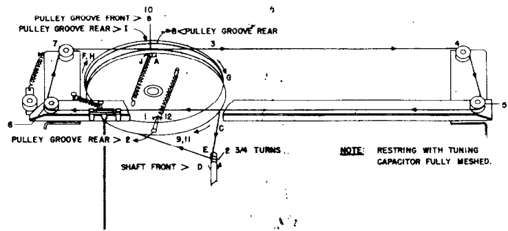
Fig. 7. Dial cable stringing procedure
