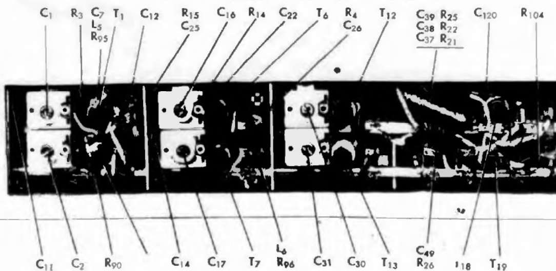
Fig. 12 Component locations, left side view.
