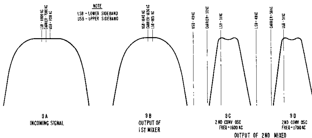
Figure 9. Selectable-Sideband Response Curves
