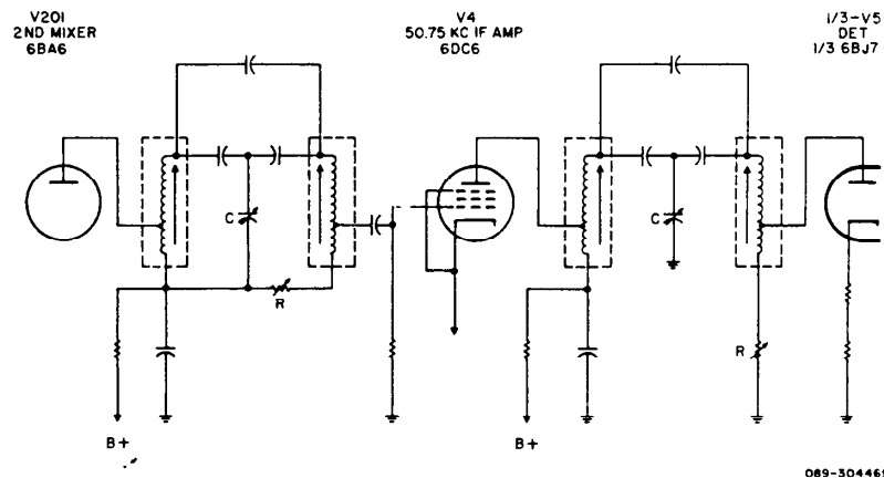
Figure 12. Equivalent Schematic Diagram of 50.75KC IF System
