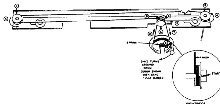
Figure 13. Dial Cord Stringing Diagram
