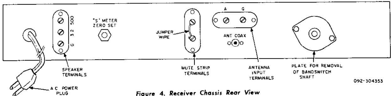
Figure 4. Receiver Chassis Rear View
