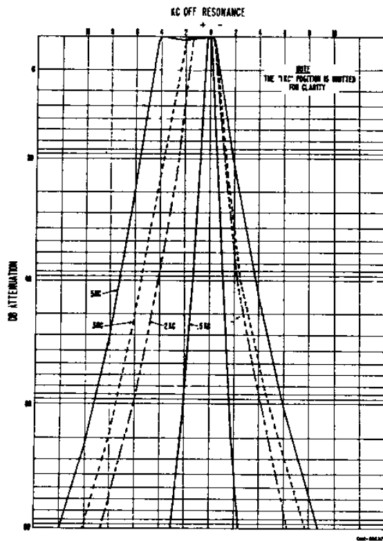
Figure 7. IF Selectivity Curves
