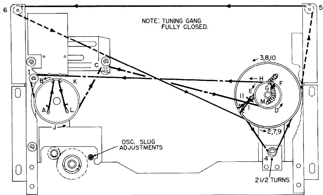
Fig. 11. Dial Pointer and Tuning Gong Stringing Diagram
