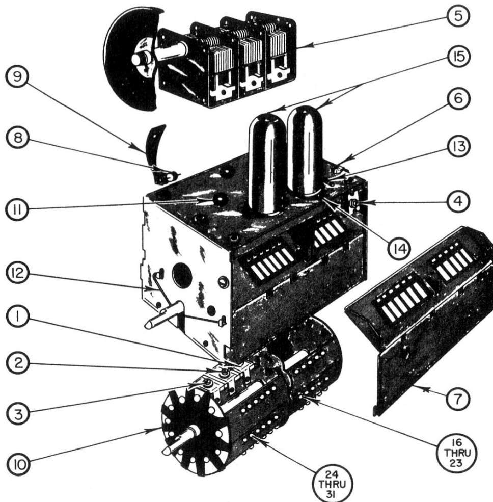
Fig. 10. Exploded View of Dynamic Turret Tuner
