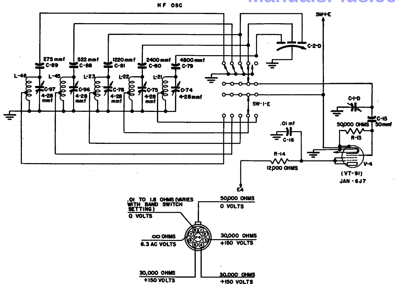
Figure 36. Radio Receiver RC-1004-C, schematic diagram of high-frequency oscillator stage.
