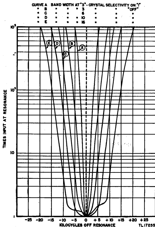
Figure 24. Selectivity chart.
