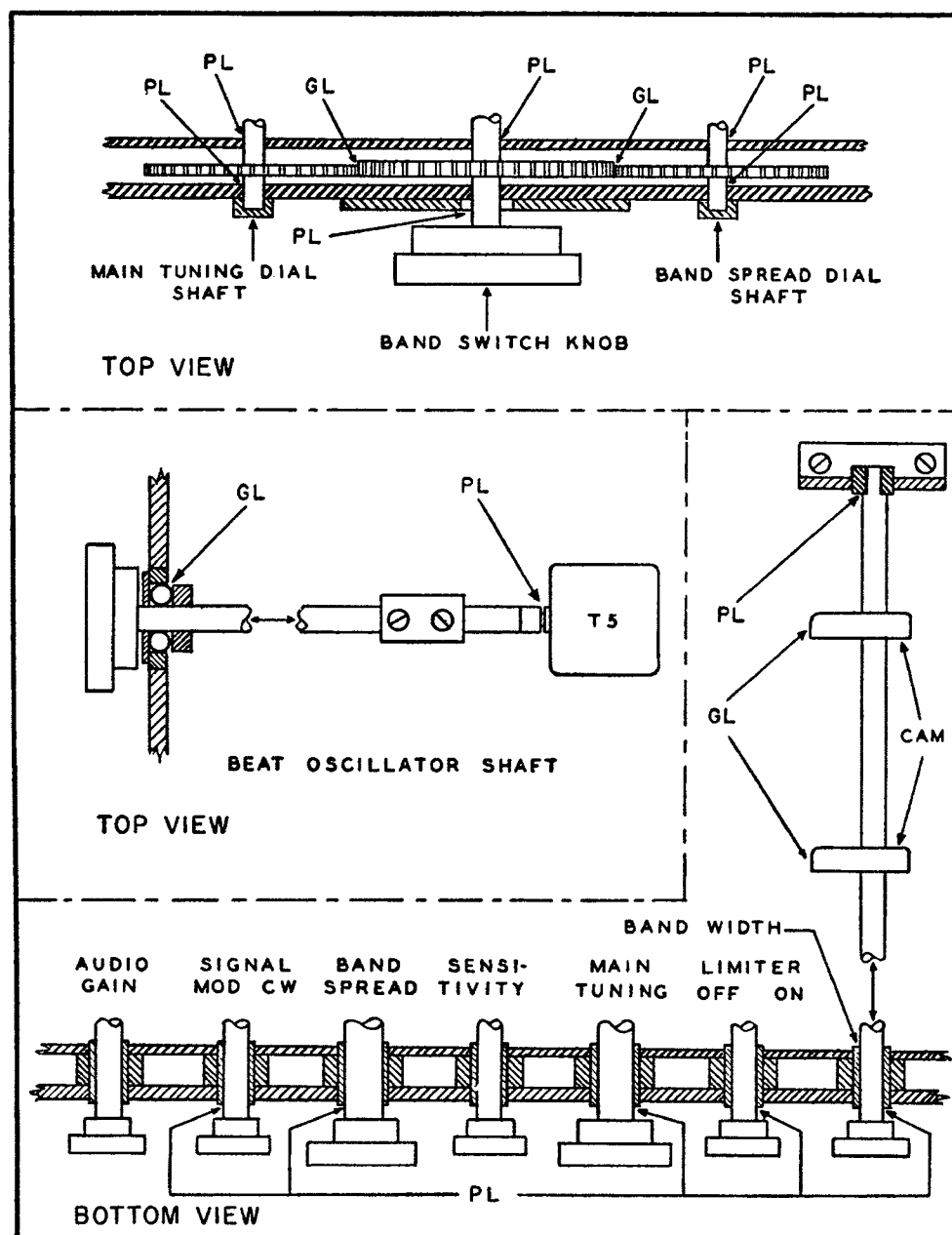
Figure 8.1 (Added.) Receiver lubrication diagram.
