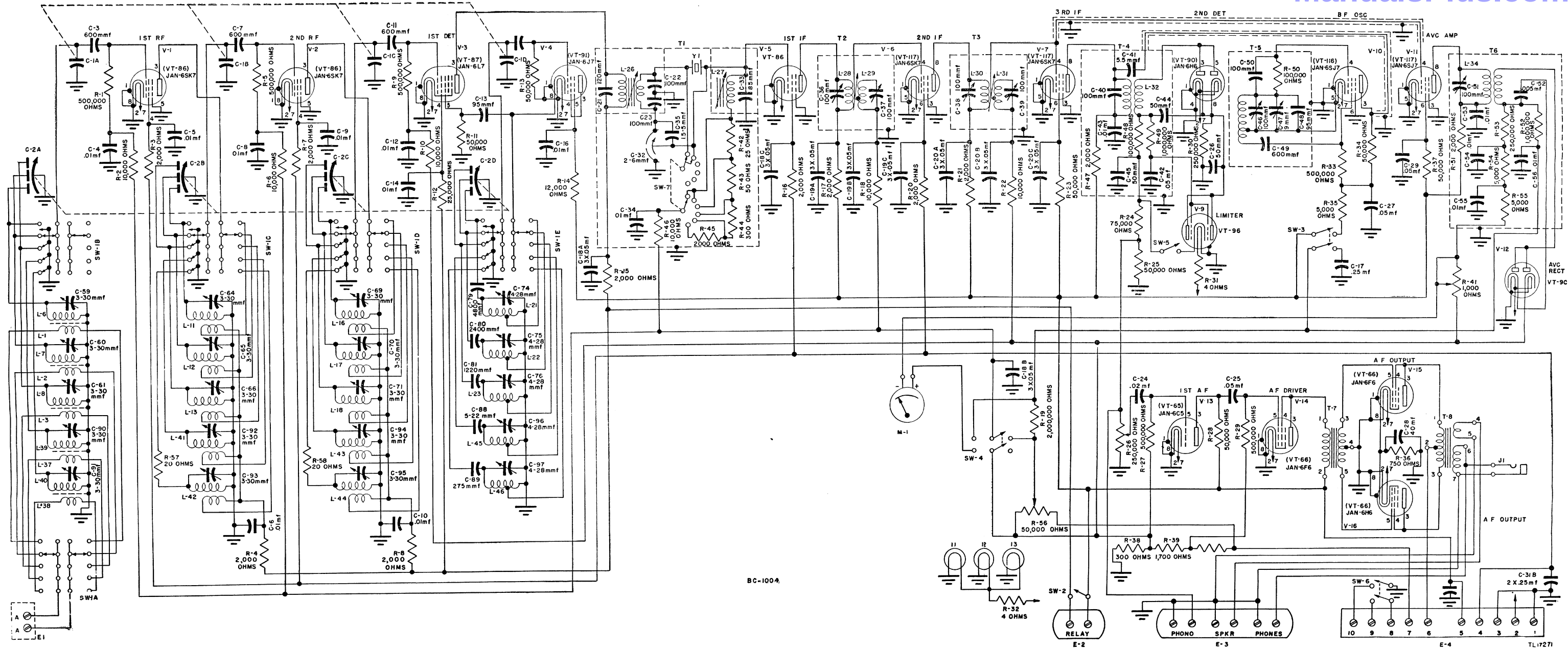
Figure 60. Radio Receiver BC-1004-C, schematic diagram.
