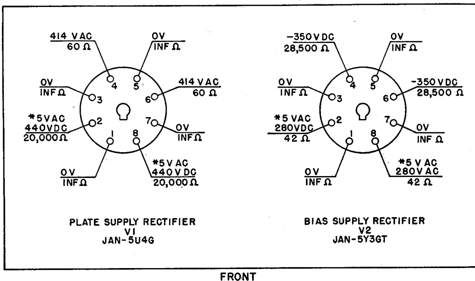
Figure 45. Power Supply Unit RA-74-D, -C, RA-84-A, -B, and RA-94-A, tube socket voltage and resistance diagram.
