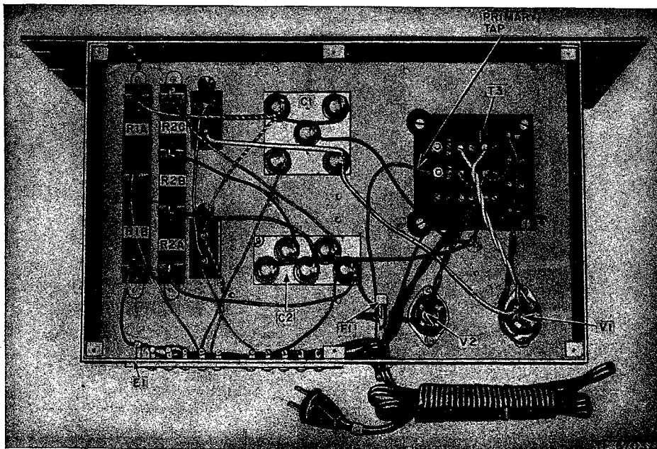
Figure 44. Power Supply Unit RA-94-A, chassis, bottom view.
