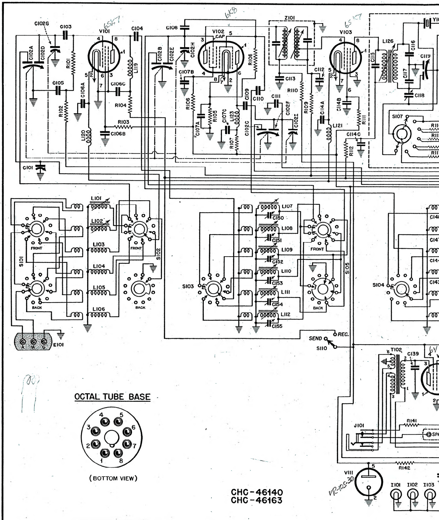
Fig. 10. Circuit Diagram—Receiver
