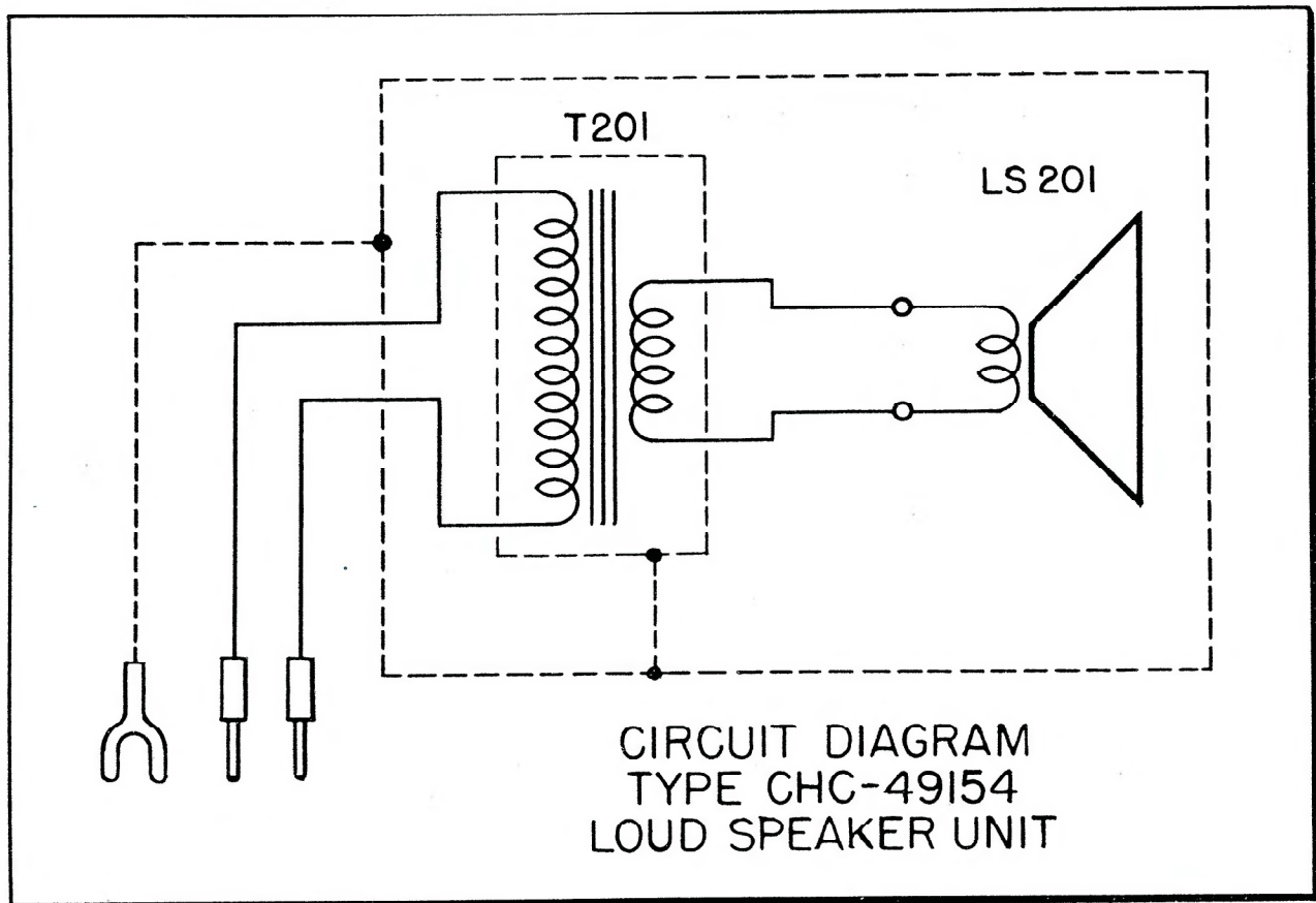
Fig. 11. Circuit Diagram—Speaker
