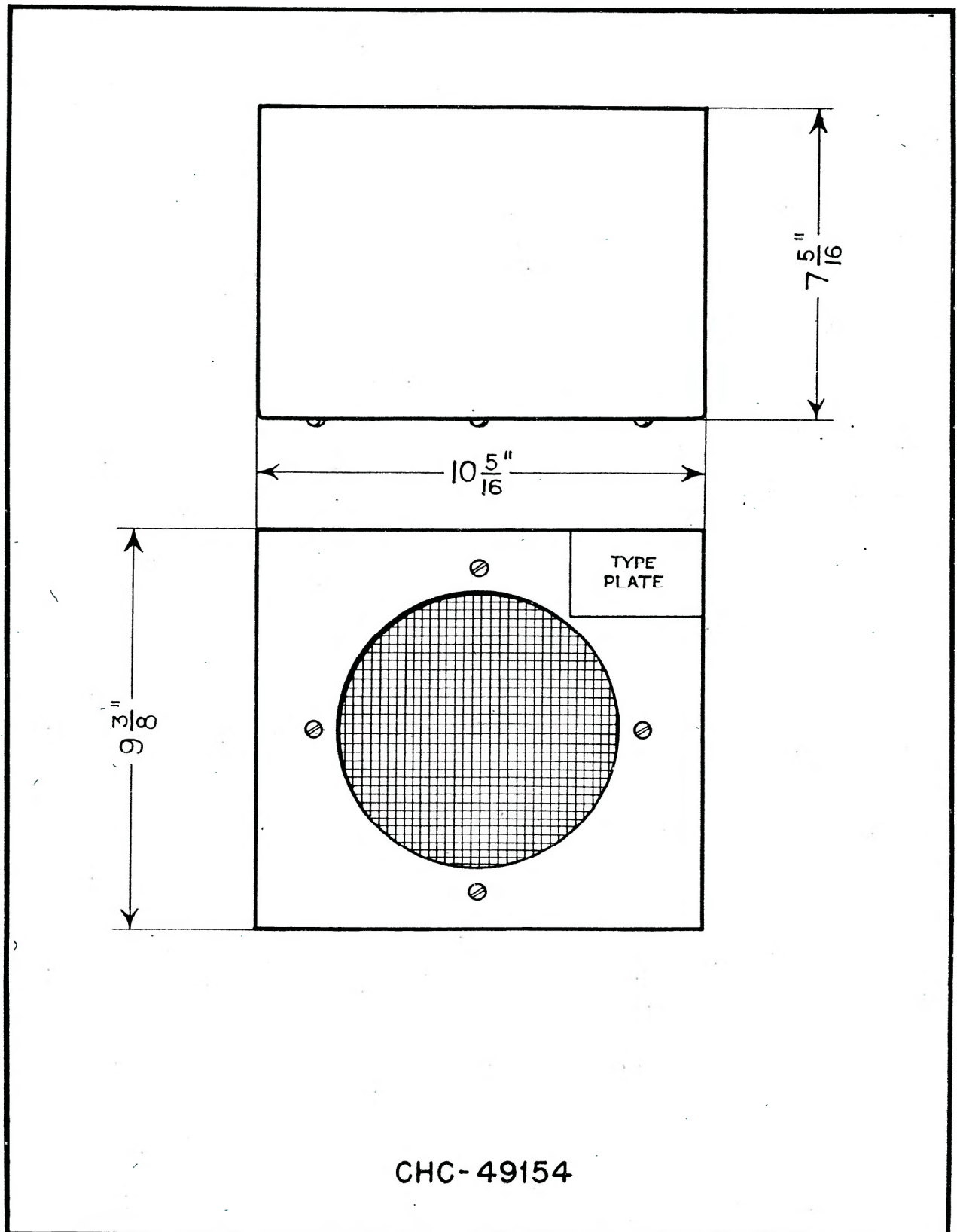
Fig. 9. Outline—Speaker
