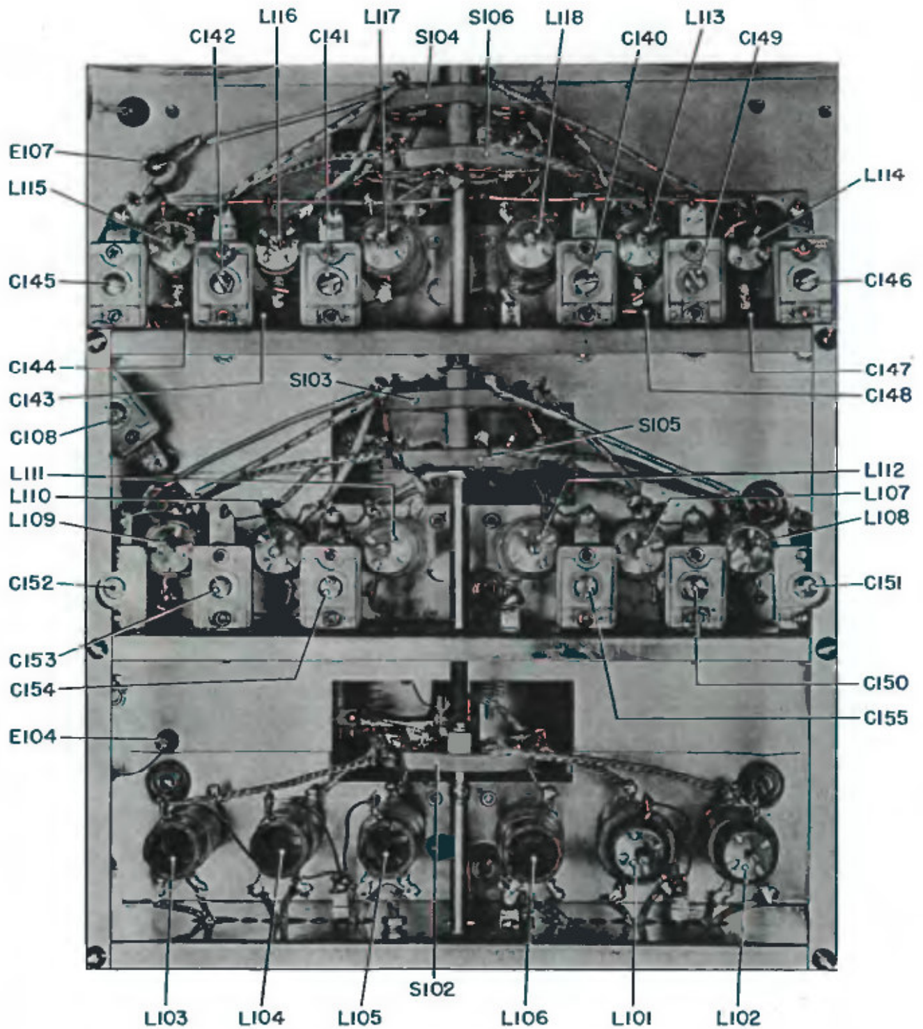
Fig. 18. RF and HF Osc. Coil Assembly
