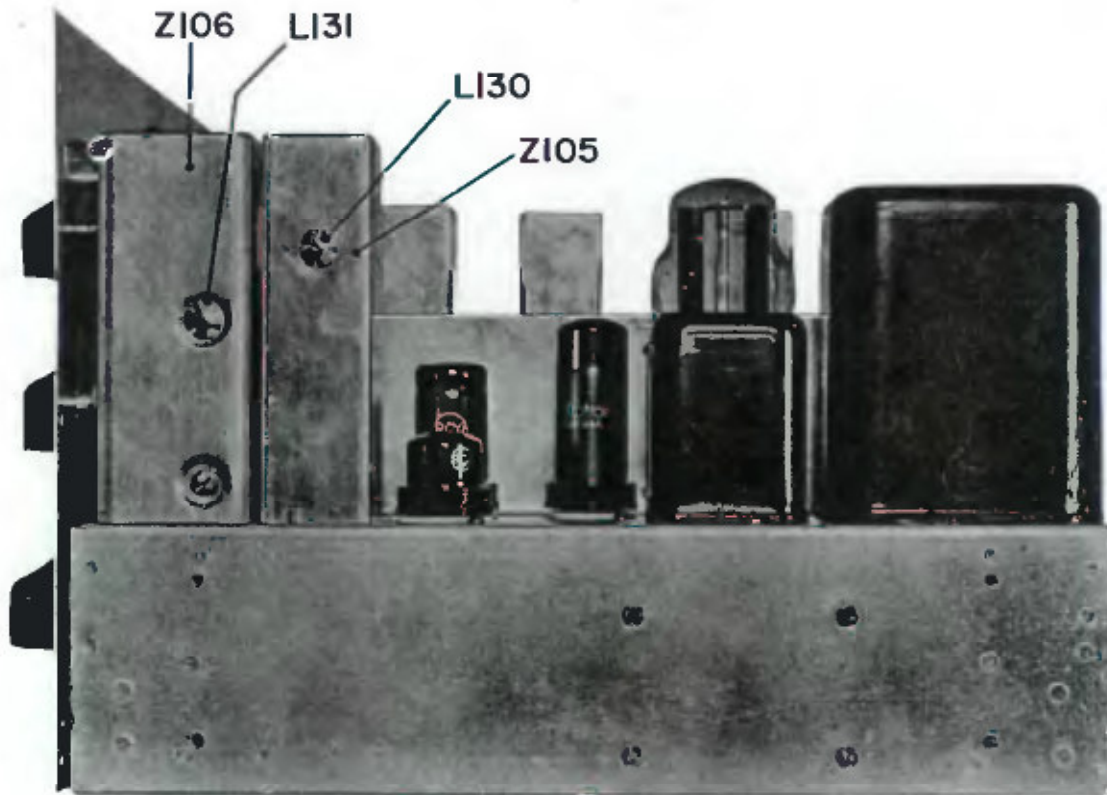
Fig. 15. Right End View of Receiver
