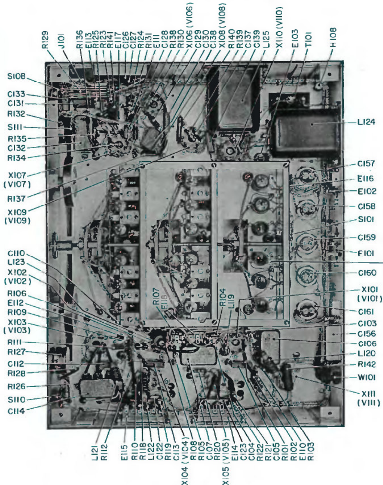
Fig. 17. Bottom View of Receiver
