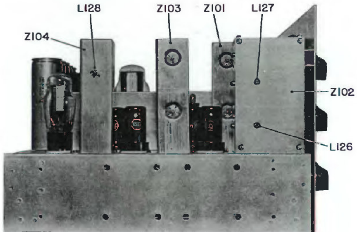
Fig. 16. Left End View of Receiver
