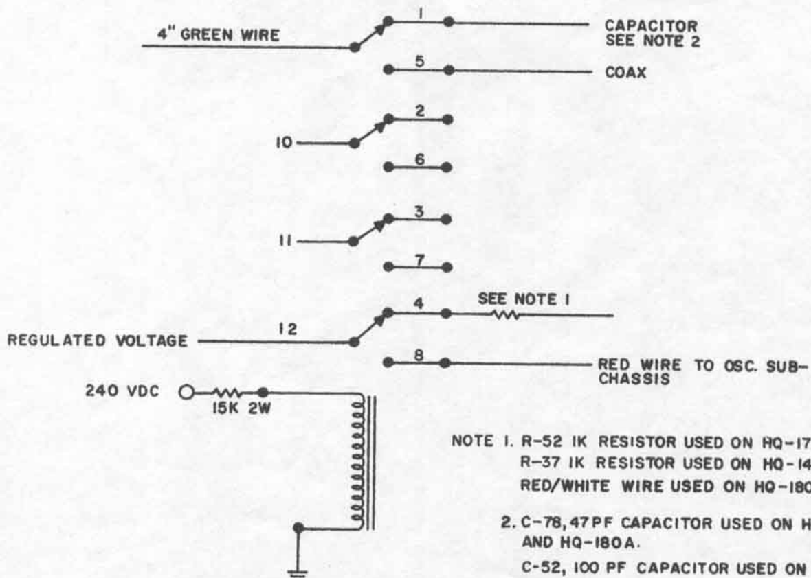
FIGURE 4. SCHEMATIC DIAGRAM OF K201 RELAY
