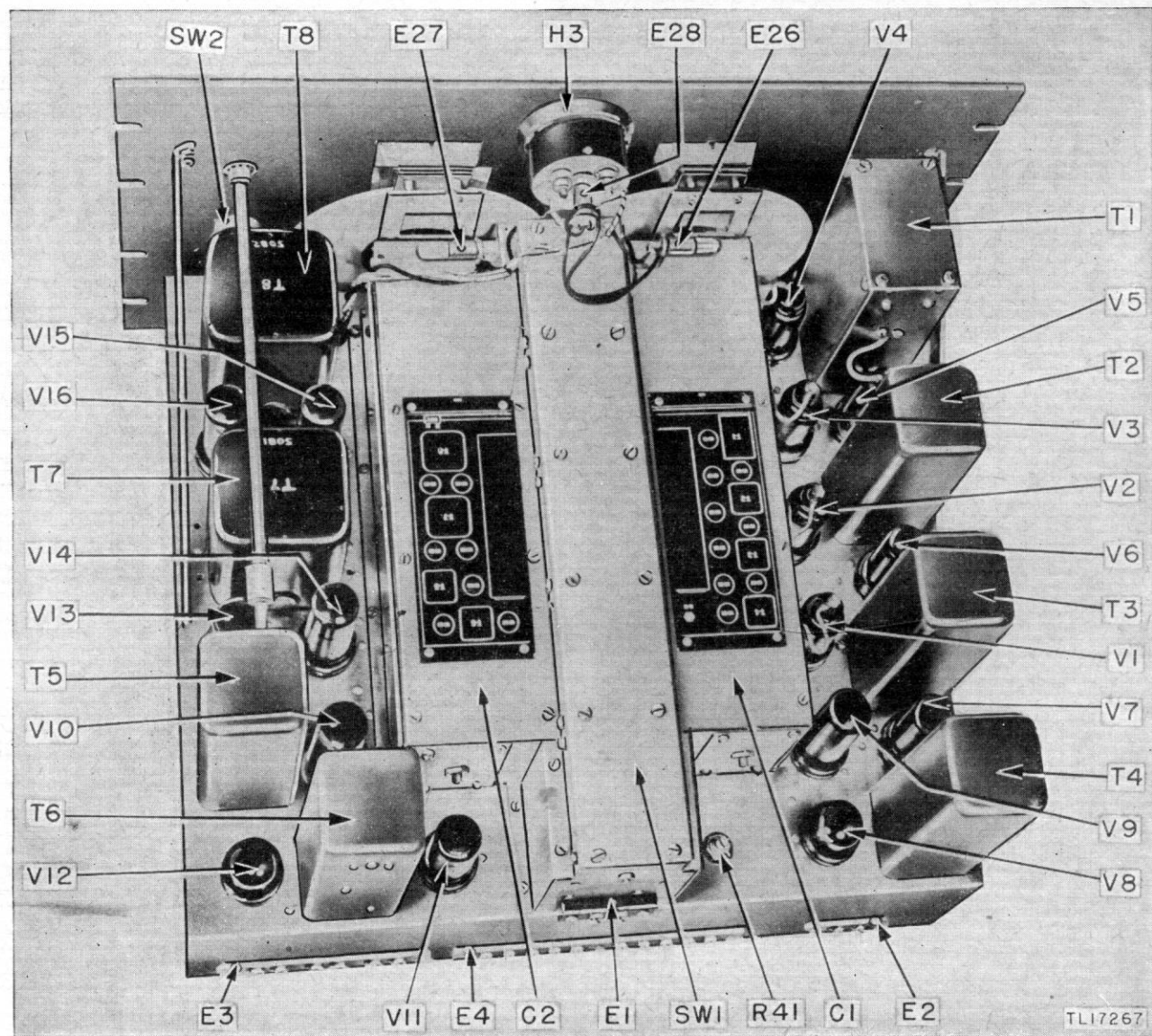
Figure 37. Radio receiver, chassis, top view.
