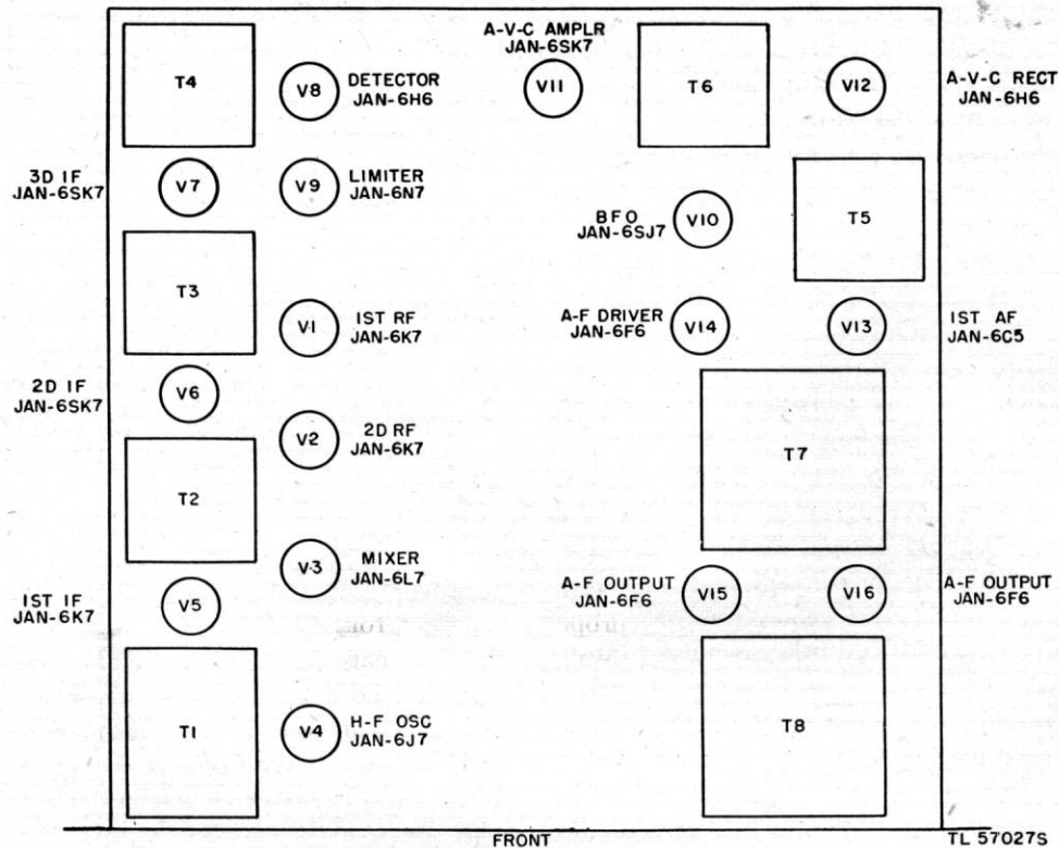
Figure 13. Radio receiver, tube location.
