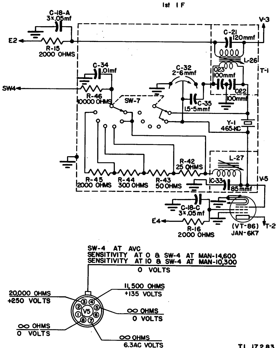
Figure 37. Radio Receivers BC-779-B, BC-794-B, and BC-1004-C, schematic diagram of first i-f stage.
