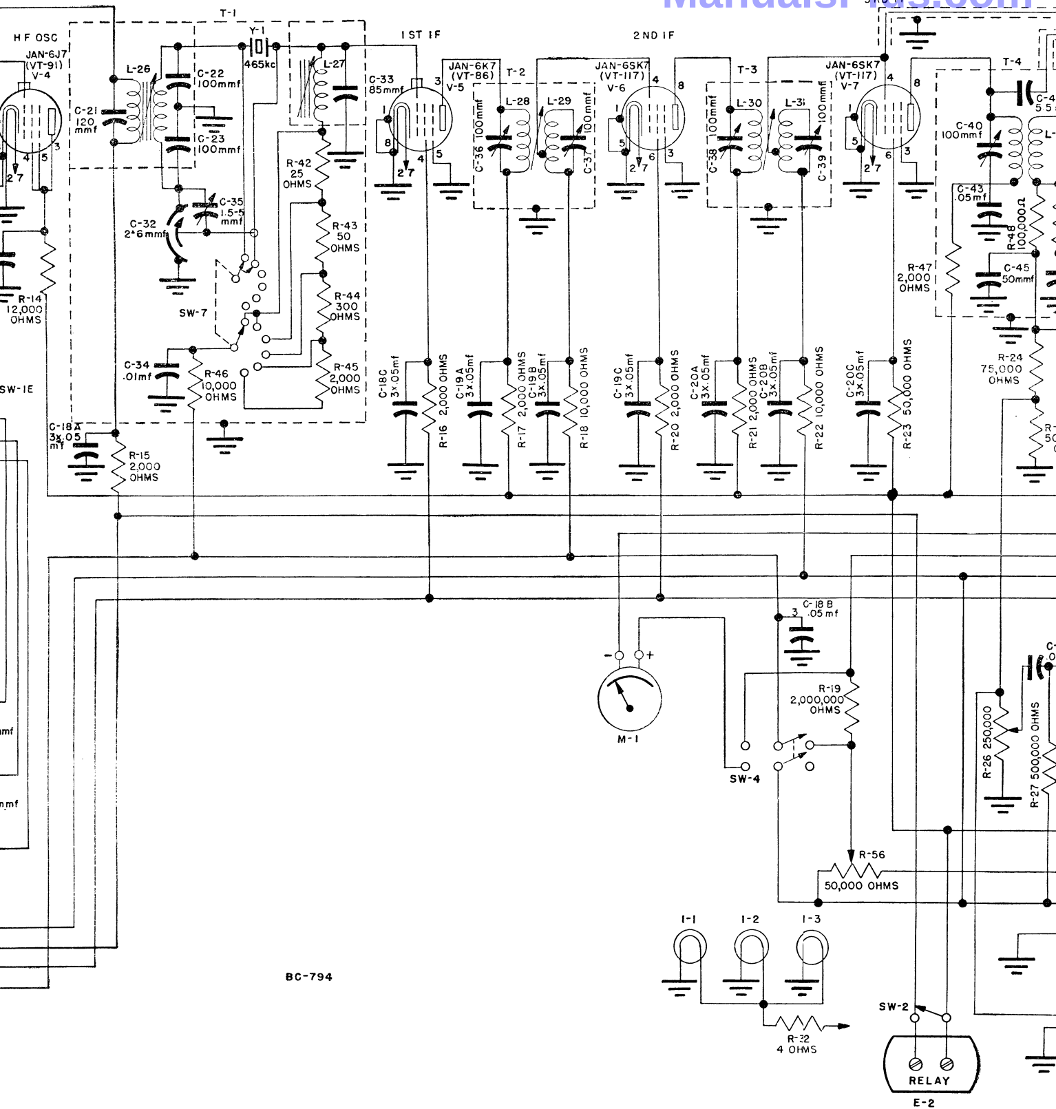
Figure 59. Radio Receiver BC-794-B, schematic diagram.
