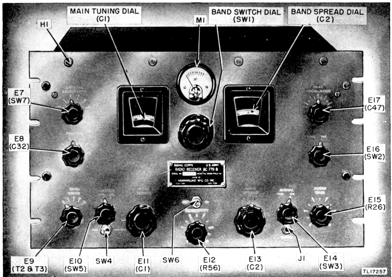
Figure 14. Radio Receiver BC-779-B, front panel parts identification.
