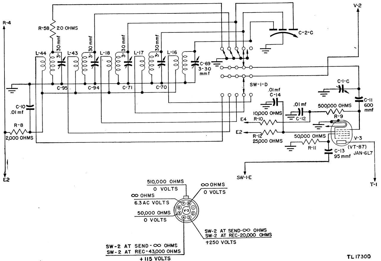
Figure 33. Radio Receiver BC-1004-C, schematic diagram of first detector stage.
