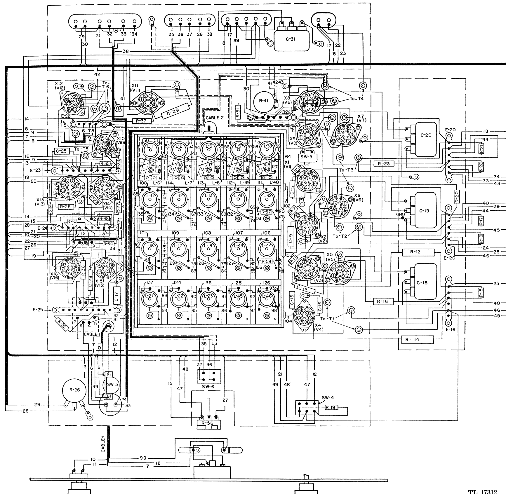
Figure 56. Chasis, pictorial wiring diagram.
