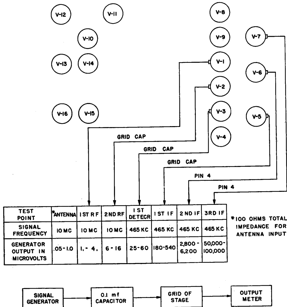
Figure 21. Signal tracing analysis chart.
