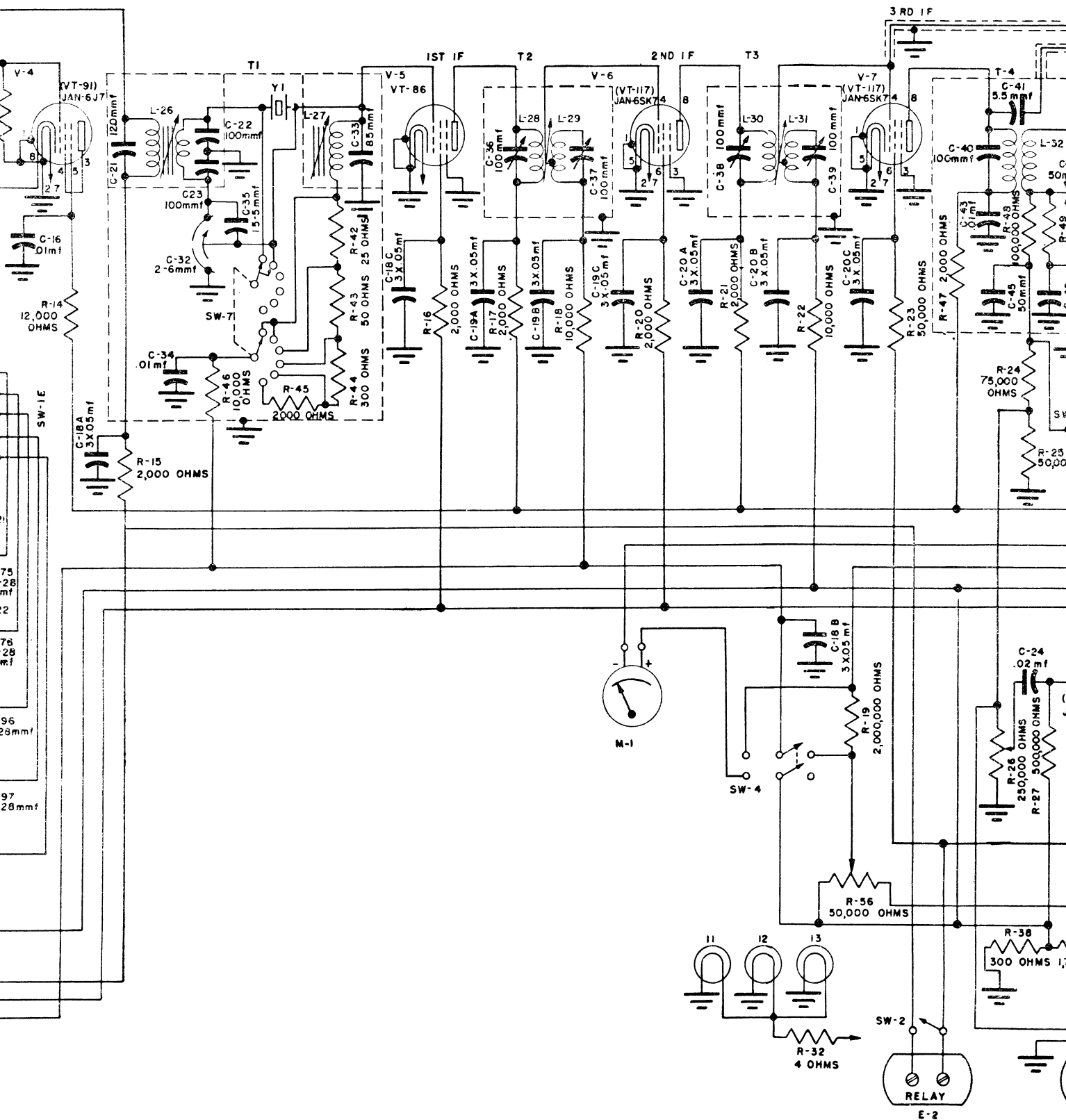
Figure 61. Radio Receiver R-129/U, schematic diagram.
