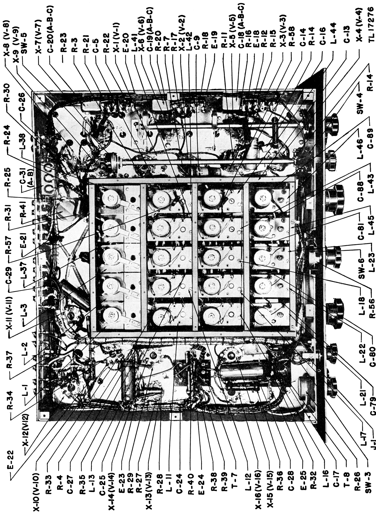
Figure 54. Radio Receiver BC-1004-C, location of parts.
