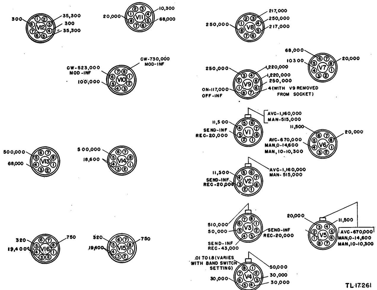
Figure 9. Tube socket resistance chart.
