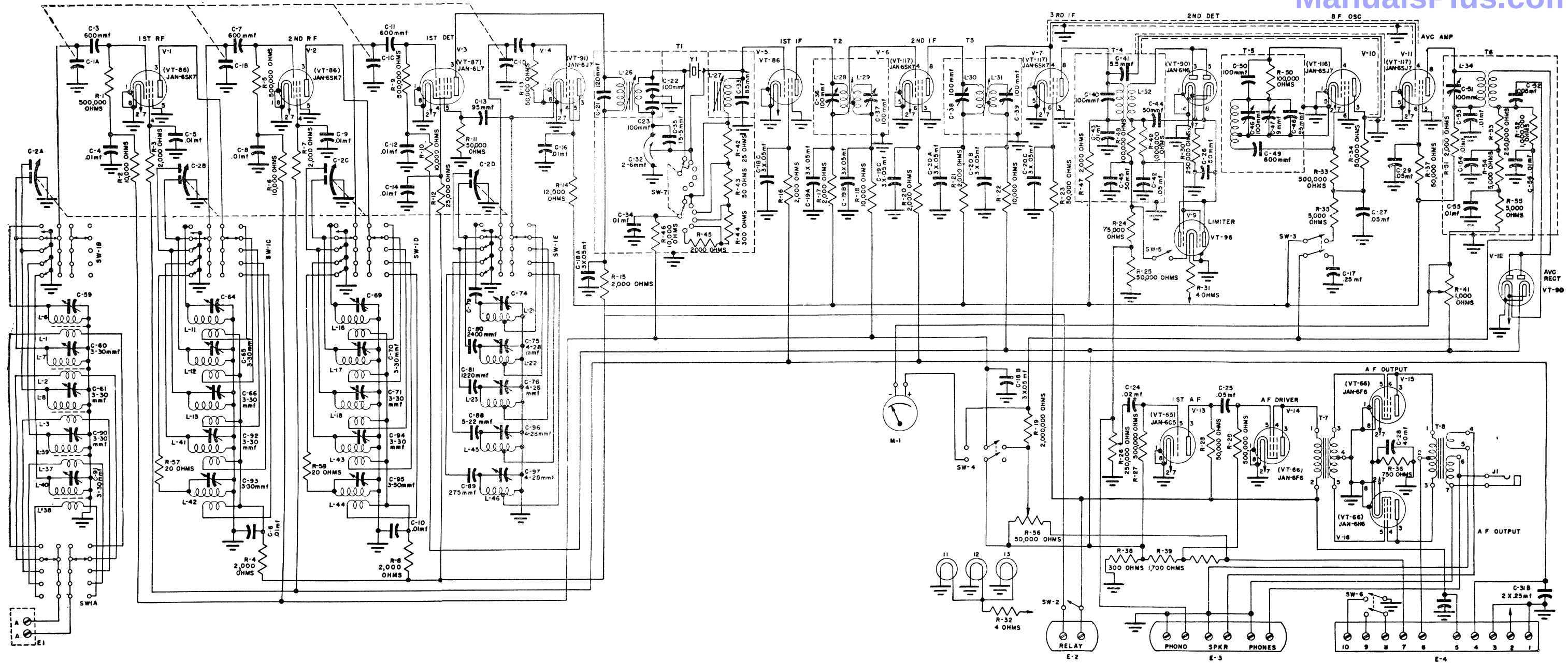
Figure 61. Radio Receiver R-129/U, schematic diagram.
