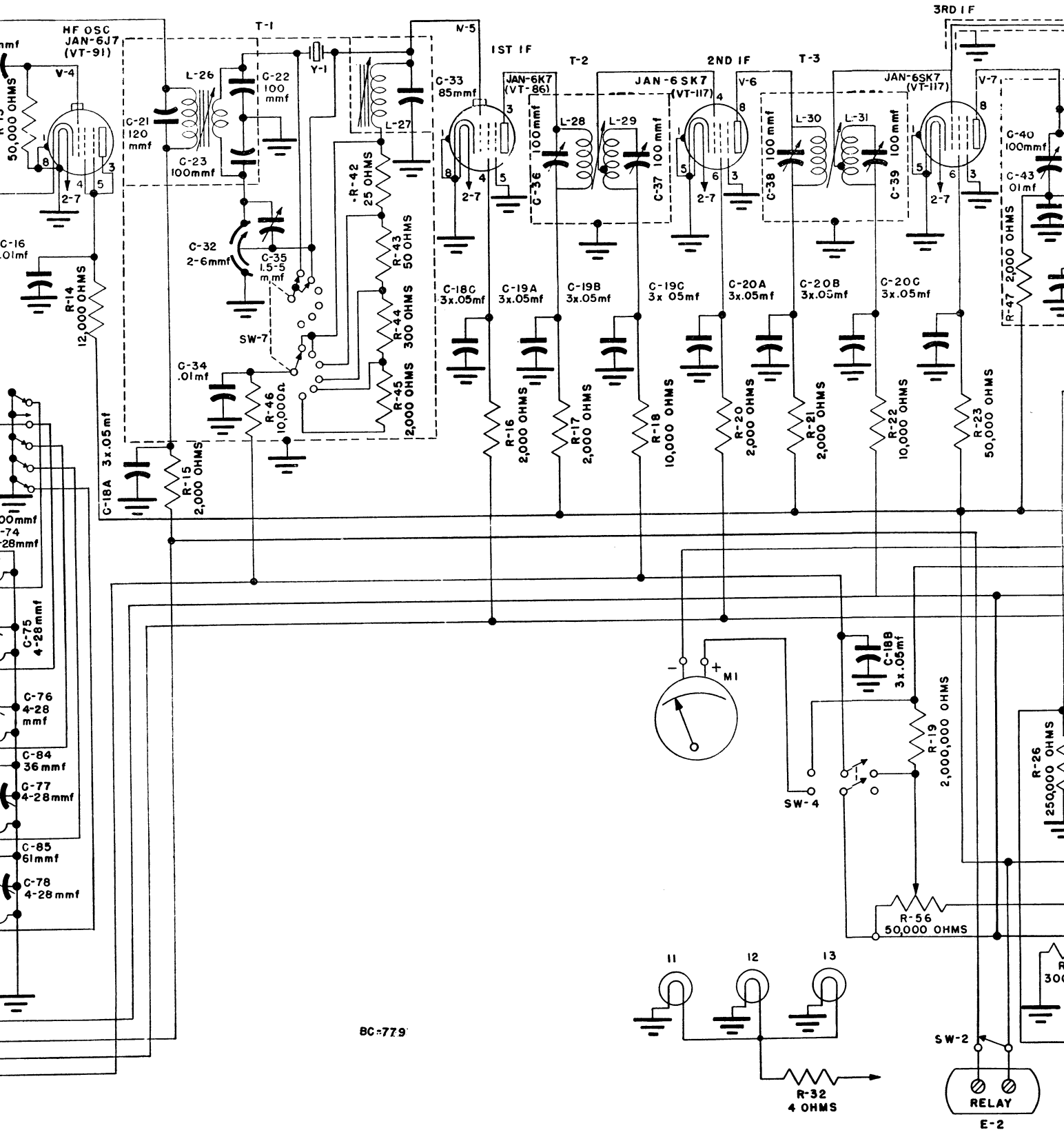
Figure 58. Radio Receiver BC-779-B, schematic diagram.
