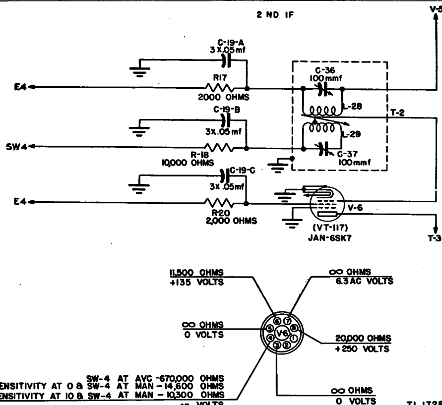
Figure 38. Radio Receivers BC-779-B, BC-794-B, and BC-1004-C, schematic diagram of second i-f stage.
