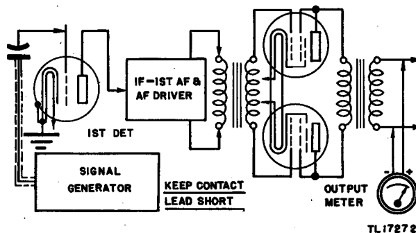
Figure 16. Typical signal generator connection diagram.
